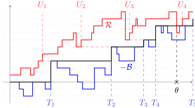
Figure 7: In red, a realization of the walk \mathcal{R} conditioned to stay positive. In blue, a realisation of the walk -\mathcal{B} and, in black, the associated process -\underline{\mathcal{B}} .
