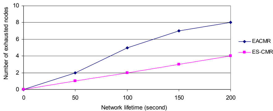
Figure 7 Number of exhausted nodes over time
