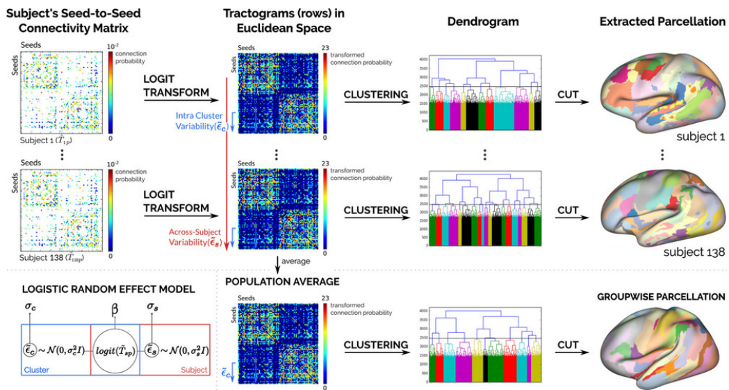
Figure 1: Lower left corner: graphical model of the linear relationship between the tractogram of a subject s for a seed p ( \tilde{T}_{sp} ); and the intra-cluster ( \tilde{\epsilon}_c ) and across-subject ( \tilde{\epsilon}_s ) variability of the seed's patch. We transform the tractograms into a Euclidean space while explicitly accounting for the variability. This allows us to use well known clustering techniques and compress different levels of granularities for a same parcellation in a dendrogram.
