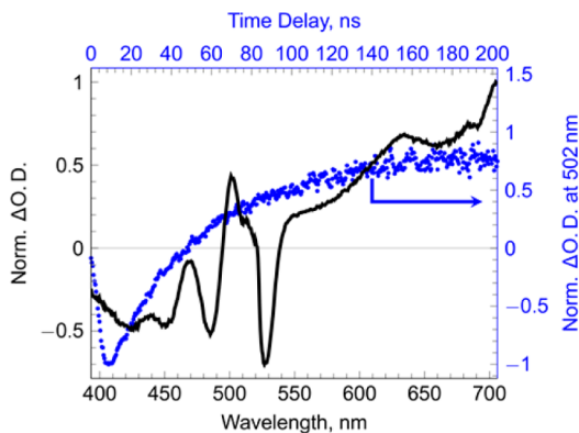
Figure 7. TRABS spectrum of OPV \text{Q}_9 PB in \text{CHCl}_3 ( \lambda_{\text{exc}} = 532 \text{ nm} , time scale 100–200 ns) and O.D. change at 502 nm.
