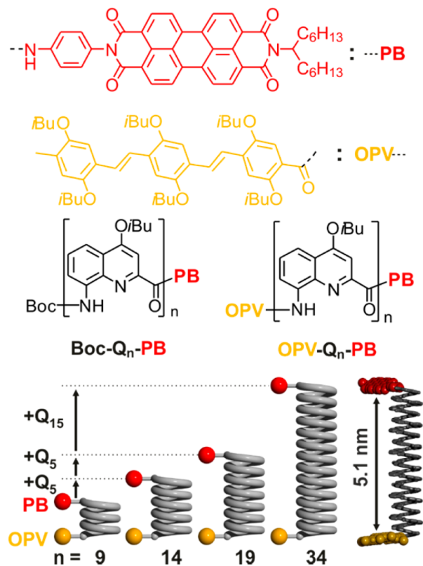
Figure 1. Formulas of studied foldamers OPV Q n PB and Q n PB. Schematic spatial representations of the helical structures of OPV Q n PB with n = 9, 14, 19, and 34 . The number of helix turns in the cartoon corresponds to the actual number expected in the molecular helix. The bottom right structure shows a color coded energy minimized (Merck molecular force field in MacroModel) model of OPV Q 34 PB. In this model, alkyl and alkoxy chains have been removed or shortened for clarity.
