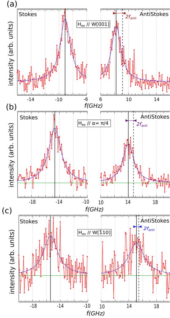
Figure 2: BLS spectra on Au/Co(0.65 nm)/W(110) with k_{SW} along the two in-plane symmetry axes. Red: experimental data. Blue line: data fit with Lorentzian functions. Green line: background fit. In the AS spectra, the distance between the continuous and dashed black lines shows the frequency shift between S and AS peaks. (a) BLS spectrum with \mu_0 H_{ext} = 0.6 T parallel to the bcc[001] axis and k_{SW} = 18.09/\mu\text{m} parallel to the bcc[\bar{1}10] axis (b) BLS spectrum with \mu_0 H_{ext} = 0.6 T along the direction with an angle of \pi/4 with respect to the bcc[\bar{1}10] axis and k_{SW} = 18.09/\mu\text{m} (c) BLS spectrum with \mu_0 H_{ext} = 0.5 T parallel to the bcc[\bar{1}10] axis and k_{SW} = 18.09/\mu\text{m} parallel to the bcc[001] axis.
