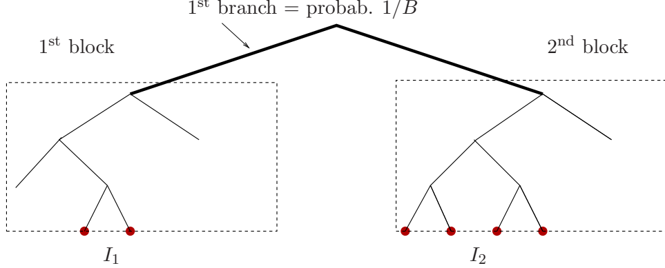
FIGURE 3. Decomposition of a non-empty complete set I into two subsets I_1 and I_2 . If I is non empty, the first generation must be non-empty (this has probability 1/B ). Conditionally on this, the occurrence of I_1 and I_2 are independent events.
