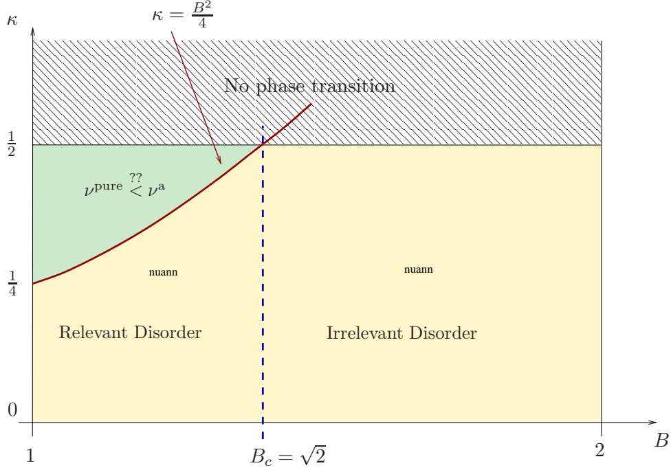
FIGURE 1. Overview of the qualitative behavior of the model. One takes \kappa < 1/2 , otherwise neither annealed nor quenched model have any phase transition. For \kappa < 1/2 \wedge B^2/4 the annealed model exhibits the same critical behavior as the pure one, and so the critical exponent is \nu^a = \nu = \log 2 / \log(2/B) . Moreover, the measures \mathbf{P}_n and \mathbf{P}_{n, h_c}^a are similar (in the sense of Proposition 3.2) and the criterion relevance/irrelevance of disorder is the same as in the i.i.d. disorder case: disorder is irrelevant for B > B_c := \sqrt{2} , marginally relevant at B = B_c and relevant for B < B_c (cf. Theorem 3.3). The region above the parabola \kappa = B^2/4 remains to be understood, but partial results (Theorem 3.6) suggest that the critical behavior of the annealed model is different from the one of the pure model, in particular the annealed critical exponent should be larger. Note that disorder is proven to be relevant for all B < B_c , \kappa < 1/2 through the “smoothing result” of Proposition 3.5, showing that the quenched critical exponent is strictly larger than the pure one.
