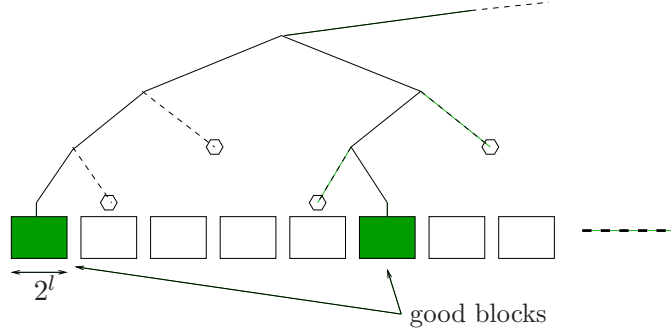
FIGURE 2. The strategy of aiming exactly at the good (colored) blocks is represented above. One first places the subtree \mathcal{T}_{\mathcal{I}}^{(n-l)} , which is present with probability (1/B)^{v(n-l,\mathcal{I})} , and then forces all the leaves that do not lead to any good block (the hexagons in the figure) not to have any children, which happens with probability larger than ((B-1)/B)^{v(n-l,\mathcal{I})} . The maximal amount of nodes that such a tree can contain is reached when all the good blocks are all equally distant one from another, and is thus bounded as in (3.19).
