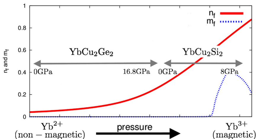
Fig. 3. Schematic comparison between the results obtained with EPAM and experiments on YbCu 2 (Si/Ge) 2 . Red solid and blue dashed lines: numerical results obtained with V = 0.1D , n_{\text{tot}} = 1.2 , U_{fc} = 0.4D , and intersite exchange J = 0.01D . E_f varies from -0.1D to -0.5D . These variations are in good agreement with experimental results either under pressure, or on replacing Si by Ge (for experimental results: see Refs. [4] and [5]).
