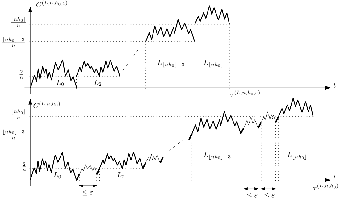
FIGURE 4. The processes C(L, n, h_0) and C(L, n, h_0, \varepsilon) .
