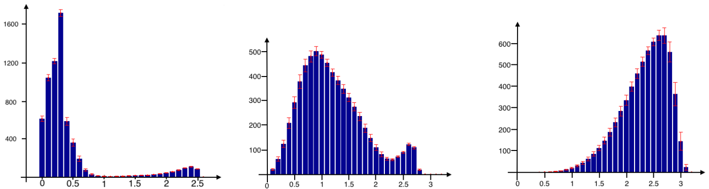
FIG. 6: Statistics for the logIPR's of all eigenstates of H for h_2 = 0.7 and different values of h_1 . From left to right: h_1 = 0.01 , h_1 = 0.07 , h_1 = 0.15 . Averages are taken over 500 realizations.
