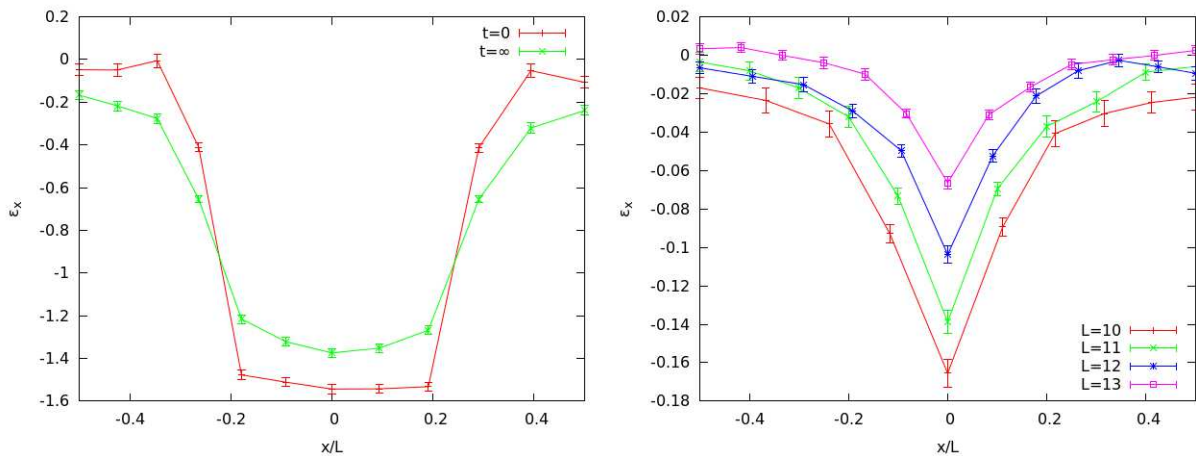
FIG. 3: Left : Disorder averaged energy per link \varepsilon_i at t=0 (red) and averaged over time (green) for L=12 . Initially a cold region of length L_c = L/2 is prepared. The disorder strength is \delta J = 3J . Right : Same protocol, but for \delta J = J and very short cold intervals ( L_c = 2 ), at various L . The memory effects diminish with increasing L , but the hot region fails to thermalize the system well, even at the largest sizes. Results were averaged over 5000 disorder realizations.
