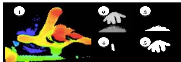
Figure 2.1. Artifacts on fingertips when fingers move very fast; 2. Initial depth map; 3 & 4. Bit-planes with a small distance from camera; 5. Bit-plane including the whole hand silhouette
