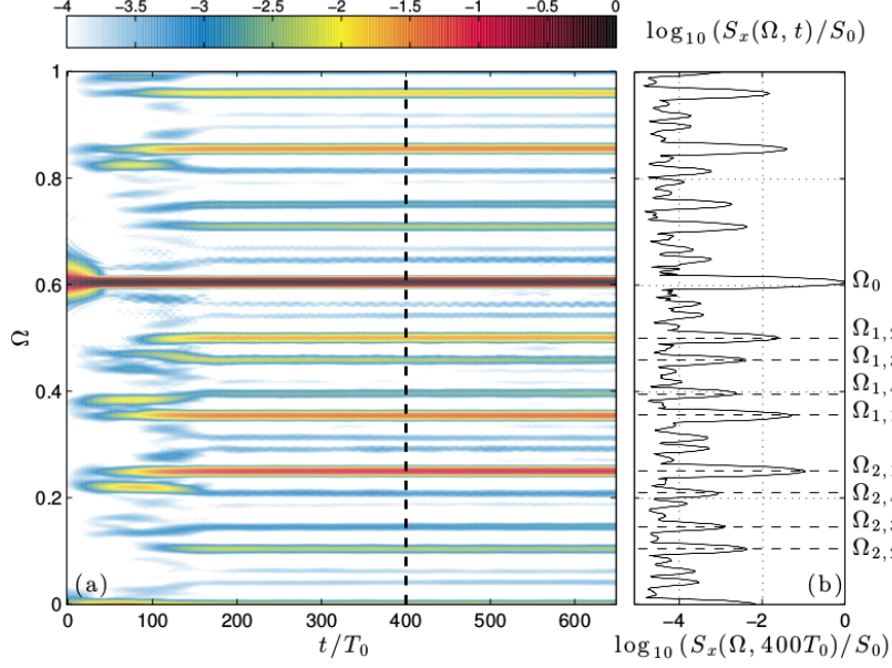
FIGURE 10. TRI cascade . (a) Time-frequency diagram of internal-wave field, obtained from a 5 \times 5 \text{ cm}^2 side square region in the most energetic wave beam; (b) Vertical cut of the diagram along the frequency axis at t = 400T_0 , indicated by the black dashed line. S_0 corresponds to the time average of the frequency component associated with the primary wave \Omega_0 . The different frequency peaks corresponding to the four first couples are labelled. Results are presented for the experiment indicated by the symbol \blacksquare in figure 4 with a=5 \text{ mm} (see Table 2 for the parameters).
