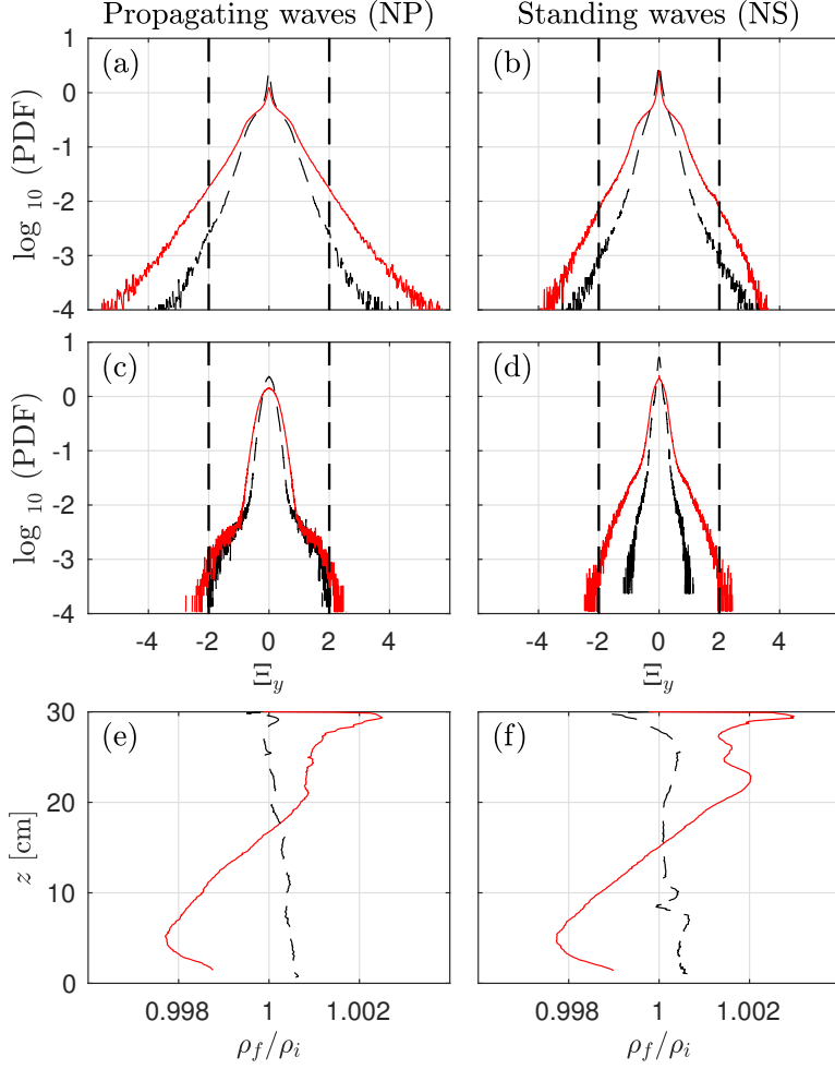
FIGURE 13. Panels (a) to (d) present the probability density functions of the vorticity in the tank, while panels (e) and (f) exhibit the ratio of the final (after 700 periods) to initial stratifications. The PDF are calculated from all images between 480 and 500 T_0 , for the two propagating (panel a, \blacksquare in figure 4) or standing (panel b, \blackstar in figure 4) wave experiments presented in figure 12. Panel (c) and (d) present the same quantity for the vorticity filtered at \Omega_0 . In all panels, dashed black and solid red lines correspond to a = 5 mm and a = 10 mm.
