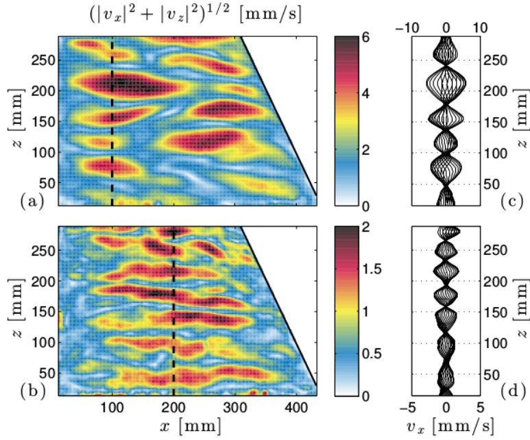
FIGURE 11. Components of the wave field corresponding to frequencies \Omega_{2,1} (a) and \Omega_{2,2} (b), obtained with the Hilbert transform around 620 T_0 using a time window 85 T_0 long. Note that the components oscillating at \Omega_{2,1} and \Omega_{2,2} correspond to standing waves as is clearly seen on the sequences of wave profiles shown on the right of each picture. Results are presented for the experiment indicated by the symbol ■ in figure 4 with a = 5 mm (see Table 2 for the parameters).
