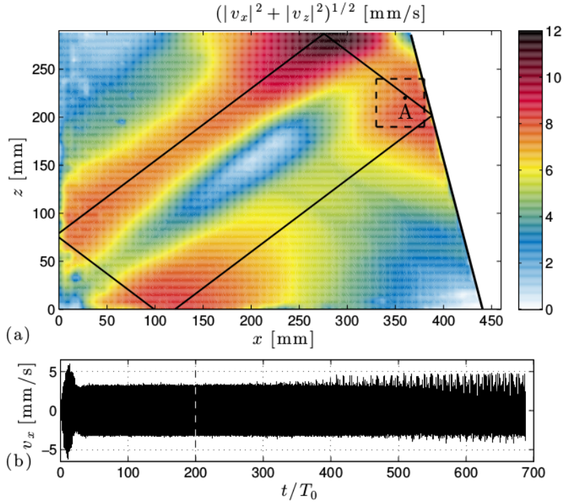
FIGURE 6. Velocity field for the experiment indicated by the symbol \star in figure 4 with a=5 mm (see Table 2 for the parameters). (a) Picture of internal wave field, filtered around \Omega_0 , 200 T_0 after the start of the wave maker and black lines show the billiard geometric prediction of the attractor. The picture presents the absolute value of the norm of the velocity vectors. The large value around the upper corner of the attractor is due to the presence of a small homogenous layer above the stratified domain. (b) the time-history of oscillations at the point A shown in (a). The vertical dashed line in (b) shows the instant of the picture (a) while the dashed square in (a) shows the region where the time-frequency diagram in figure 7 has been calculated. The initial transient is due to the setting of the attractor, while the instability is noticeable after roughly 400 periods of oscillations.
