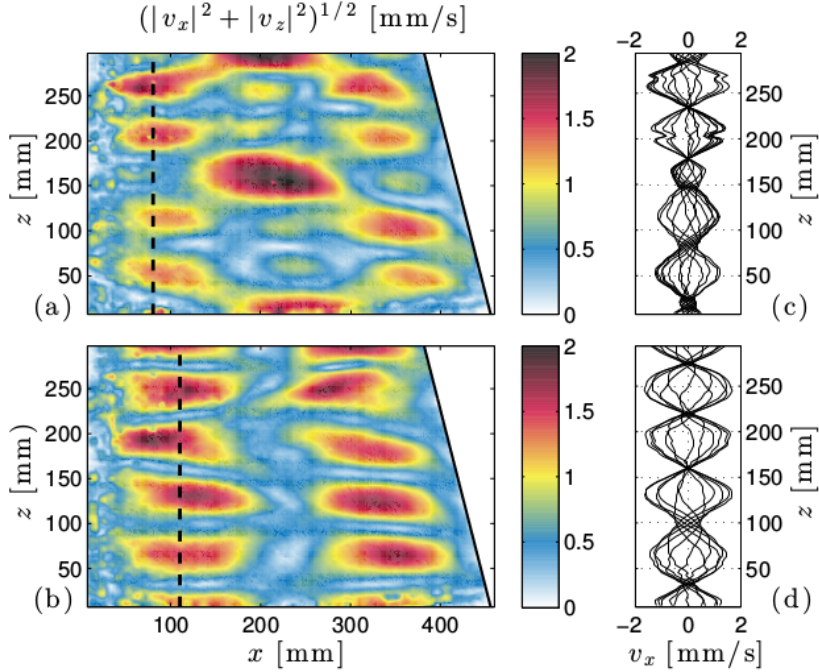
FIGURE 8. Components of the wave field corresponding to frequencies \Omega_1 (panel a) and \Omega_2 (panel b), obtained with the Hilbert transform around 620 T_0 using a time window 85 T_0 long. Results are presented for the experiment indicated by the symbol \star in figure 4 with a=5 mm (see Table 2 for the parameters). Note that the components oscillating at \Omega_1 and \Omega_2 correspond to nearly standing waves as is clearly seen on the sequences of wave profiles shown on the right of each picture.
