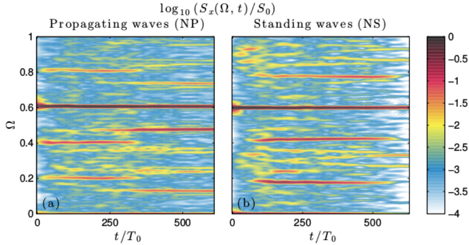
FIGURE 12. Time-frequency diagrams of two signals recorded in unstable wave attractors corresponding to different operating points. Both attractors are unstable and the wave regime is such that it induces significant mixing. The left panel corresponds to the experiment indicated by the symbol \blacksquare in figure 4, while the right one by the \star (with a = 10 mm and other parameters listed in Table 2).
