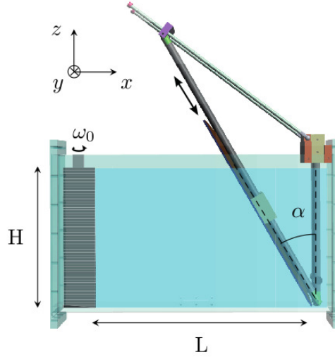
FIGURE 2. Sketch of the experimental set-up showing the wave generator and the sloping wall (inclined at an angle \alpha with respect to the vertical) inside the immobile tank of size 800 \times 170 \times 425 \text{ mm}^3 . The working bottom length of the section, the depth and the sloping angle are given within the text.
