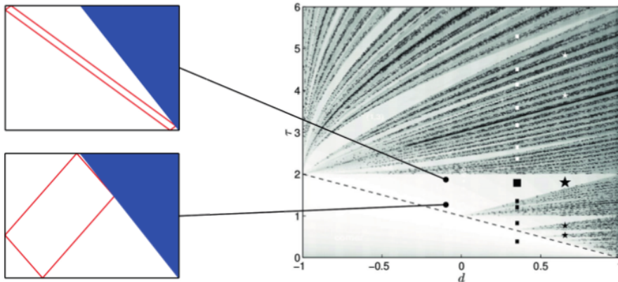
FIGURE 1. Right panel presents the (d, \tau) diagram obtained by Maas et al. (1997). Left panels present two examples of the corresponding (1, 1) attractor. The different symbols in the right panel correspond to the different peak frequencies for the 2 experiments ( \blacksquare and \star in Table 2 with a = 5 mm). The primary wave frequency is plotted with a filled and larger symbol. The subharmonics (respectively superharmonics) are represented by white (respectively black) symbols.
