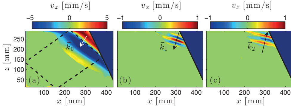
FIGURE 5. Horizontal velocity fields for the experiment indicated by the symbol \blacksquare in figure 4 and Table 2 for a = 5 mm, filtered at \Omega_0 (panel a), \Omega_1 (panel b) and \Omega_2 (panel c) in frequency and in space to keep only the relevant directions. The velocity field is displayed only where the wave amplitude is larger than 15% of the maximum. The wave vectors are represented by the arrows. Black dashed lines show the billiard geometric prediction of the attractor.
