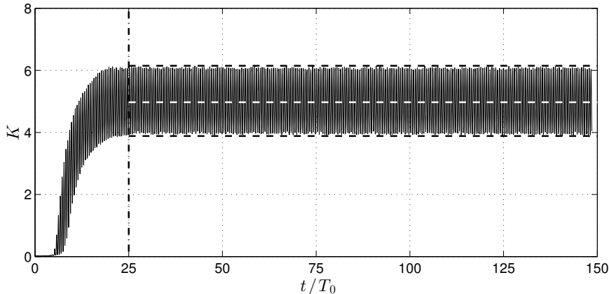
FIGURE 3. Typical experimental time-history of the nondimensional kinetic energy. The vertical dotted dashed line indicates the instant where the kinetic energy saturates. The average of the signal, computed from this instant and to the end of the experiment, is represented by the dashed white line. The two horizontal dashed black lines represent K_{min} and K_{max} , the minimal and maximal values bounding the oscillations of the kinetic energy during the saturated state. The parameters for this experiment are: \Omega_0=0.59 , H=300 mm, L=450 mm, \alpha = 27.3^\circ , \tau = 1.84 , d = 0.31 and a = 1.5 mm. For this experiment, \langle K \rangle = 5 and R = 0.65 .
