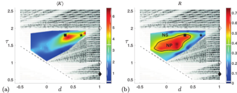
FIGURE 4. Structure of Arnold tongue of a stable (1, 1) attractor in terms of the mean normalized kinetic energy \langle K \rangle (panel a) and the ratio of minimum to maximum kinetic energy R (panel b). The results are plotted from the 50 experiments described in Table 1. Superimposed on this picture are three different symbols corresponding to the location of the three main long-term experiments discussed throughout this paper: \blacklozenge and \diamond for the case of the rectangular domain discussed by McEwan (1971) (see § 4.1), \blacksquare for the well-focused (1, 1) attractor discussed in Brouzet et al. (2016a) with propagating waves (see § 4.2), \blackstar for the weakly-focused (1, 1) attractor described here (see § 4.3). The solid black line shows the contour at the value R = 0.5 , enclosing the region with nearly propagating waves (NP), while nearly standing waves (NS) are outside this region.
