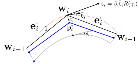
Fig. 4: Illustration of the interpolation process using quintic Bézier curves. The blue line is the first computed piecewise linear path. The red dashed line is the smoothed path using quintic Bézier curves.
