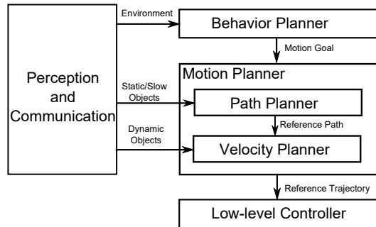
Fig. 2: Autonomous driving architecture: a simplified view
