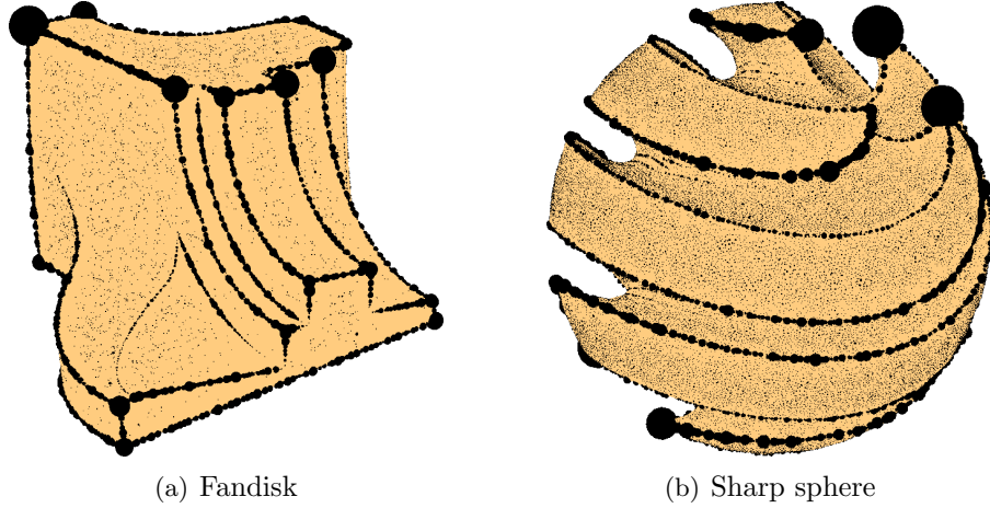
Figure 3: Convolved boundary measures of 100k point clouds sampled from the fandisk and sharp sphere models and rescaled so as to have unit diameter. The offset radius is set to r = 0.05 and r = 0.1 respectively and the convolution radius is given by \varepsilon = 0.02 and \varepsilon = 0.03 .
