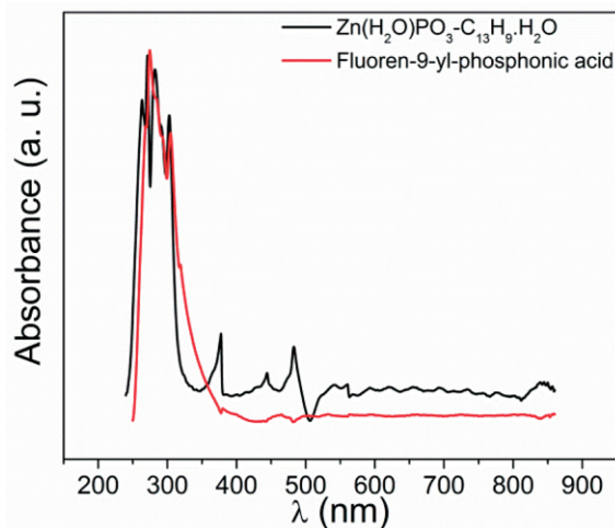
Figure 5. Normalized absorbance with baseline correction of Zn(H_2O)PO_3-C_{13}H_9\cdot H_2O (black line) and fluorene-9-yl-phosphonic acid (red line) samples, obtained from specular transmittance measurement on powder.
