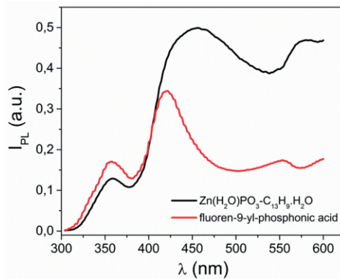
Figure 6. Photoluminescence spectra of Zn(H_2O)PO_3-C_{13}H_9\cdot H_2O stacked between two quartz suprasil glass slides (black line) and of a fluorene-9-yl phosphonic acid single crystal (red line). Excitation line: 266 nm, power density of 23.5 \text{ mW}\cdot\text{mm}^{-2} , 900 gratings per mm, frequency of 9 Hz for Zn(H_2O)PO_3-C_{13}H_9\cdot H_2O and 8.95 Hz for fluorene-9-yl phosphonic acid.
