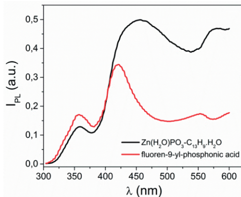
Figure 6. Photoluminescence spectra of Zn(H_2O)PO_3-C_{13}H_9\cdot H_2O stacked between two quartz suprasil glass slides (black line) and of a fluoren-9-yl phosphonic acid single crystal (red line). Excitation line: 266 nm, power density of 23.5 \text{ mW}\cdot\text{mm}^{-2} , 900 gratings per mm, frequency of 9 Hz for Zn(H_2O)PO_3-C_{13}H_9\cdot H_2O and 8.95 Hz for fluoren-9-yl phosphonic acid.
