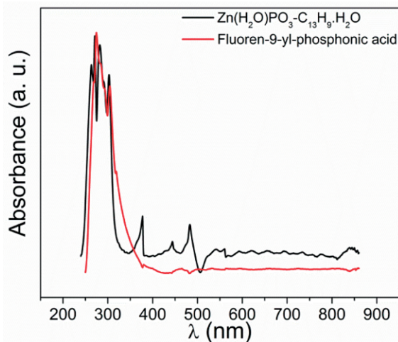
Figure 5. Normalized absorbance with baseline correction of Zn(H_2O)PO_3-C_{13}H_9\cdot H_2O (black line) and fluoren-9-yl-phosphonic acid (red line) samples, obtained from specular transmittance measurement on powder.
