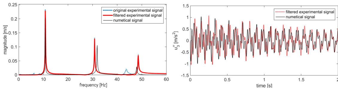
Figure 4. Experimental and numerical top floor response
