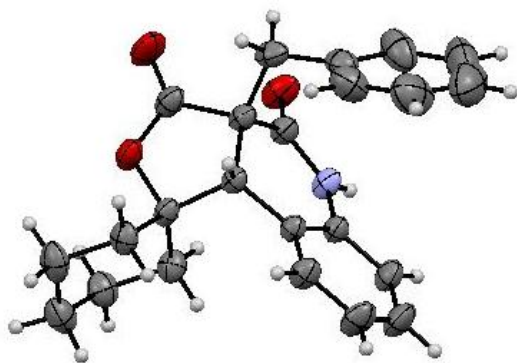
Figure 3. ORTEP view of one enantiomer of (\pm) 10a
