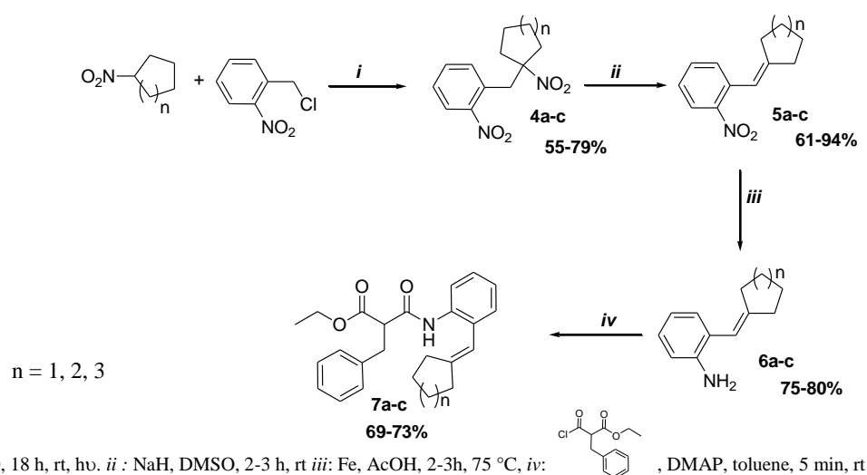
Scheme 3. Synthesis of starting materials 7a-c
