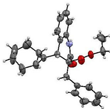
Figure 2. ORTEP view of one enantiomer of (\pm) 9c
