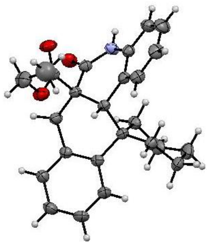
Figure 1. ORTEP view of one enantiomer of (\pm) 8a
