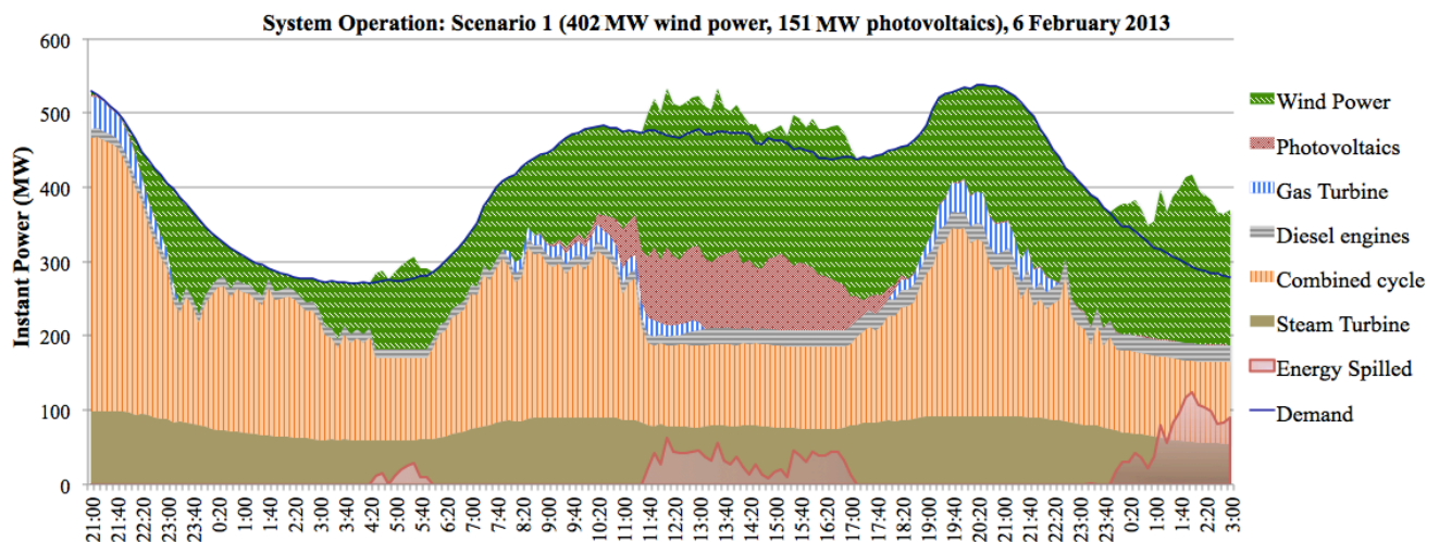
Figure 3. Winter operation of the system (Scenario 1, 402 MW wind power and 151 MW photovoltaic). 6 February 2013.
