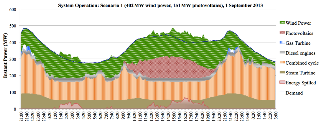
Figure 4. Summer operation of the system (Scenario 1, 402 MW wind power and 151 MW photovoltaic). 1 September 2013.
