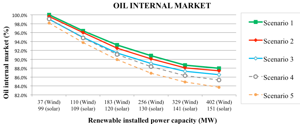
Figure 10. Oil internal market. (a) Scenario 1 (baseline); (b) Scenario 2 (10,000 EVs); (c) Scenario 3 (25,000 EVs); (d) Scenario 4 (25,000 EVs using V2G) and (e) Scenario 5 (50,000 EVs using V2G).
