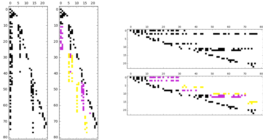
Figure 2: Support of the matrices C = LQ (left), E = PU (top right) of the s -overlapping CRE decomposition of Theorem 19 applied to the matrix of Figure 1. The Compression to the block bi-diagonal structure of the corresponding compact Bruhat generator is shown in the central and bottom right matrices. There, D is in black and S in magenta and yellow; those rows and columns moved at step 10 of Algorithm 3 are in yellow.
