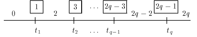
Figure 2: Zones defined by a q -interval
