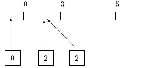
Figure 5: Composing (0, 2, 2) with (0, 3, 5)
