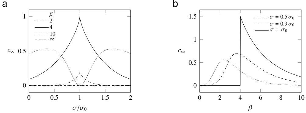
Figure B.27: Specific heat in the thermodynamic limit as function of the loading (a) and as function of temperature (b). Here, v_0 = 1 .
