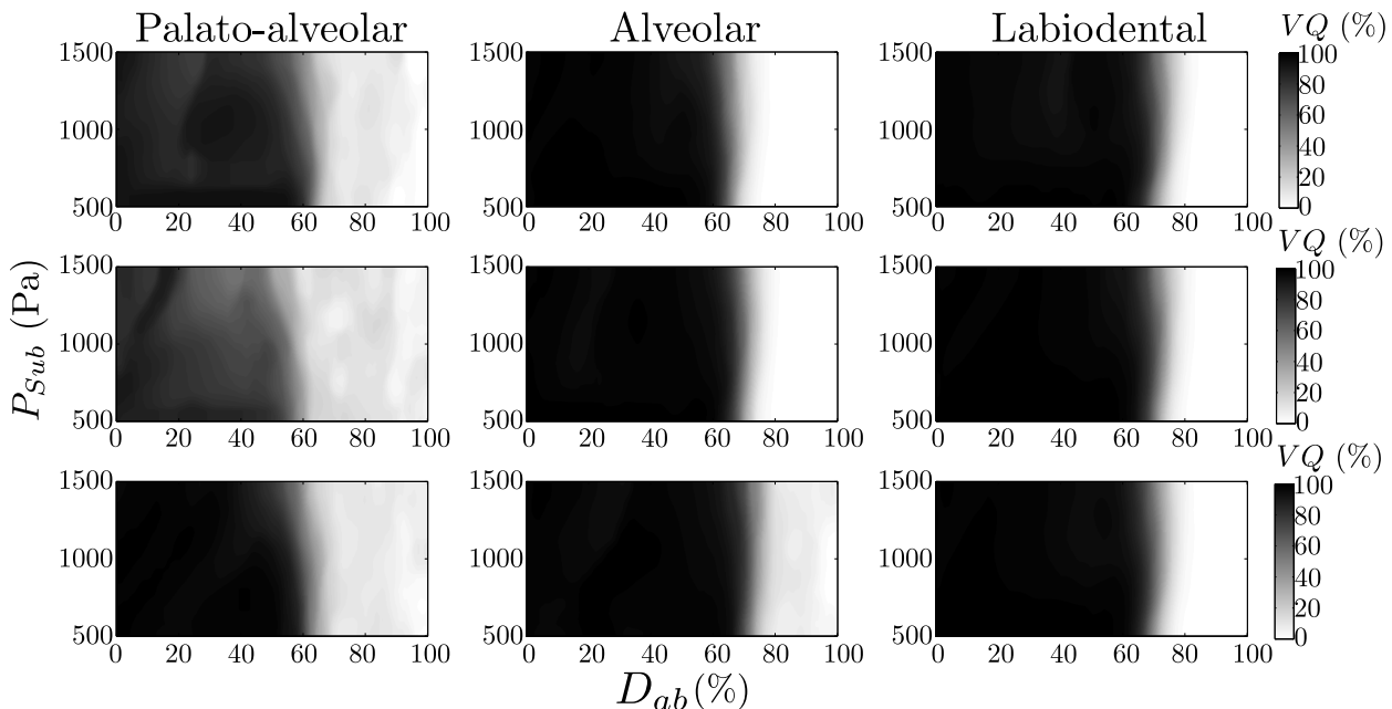
Figure 5. Voicing quotient of simulated voice signals as a function of the subglottal pressure P_{Sub} and the glottal abduction degree D_{ab} . Each column of figures corresponds to a place of articulation. From left to right: palato-alveolar fricatives / \text{ʃ}, \text{ʒ} /, alveolar fricatives / \text{s}, \text{z} /, and labiodental fricatives / \text{f}, \text{v} /. Each row of figures corresponds to a vowel context, / \text{i}, \text{a}, \text{u} /, from top to bottom.
