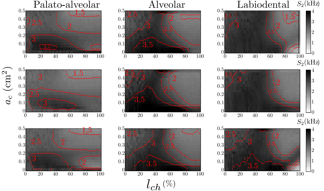
Figure 10. Spectral spread of simulated voice signals as a function of the supraglottal constriction area a_c and the glottal chink opening l_{ch} . Each column of figures corresponds to a place of articulation. From left to right: palato-alveolar fricatives /\text{ʃ}, \text{ʒ}/ , alveolar fricatives /\text{s}, \text{z}/ , and labiodental fricatives /\text{f}, \text{v}/ . Each row of figures corresponds to a vowel context, /\text{i}, \text{a}, \text{u}/ , from top to bottom. Contour lines, expressed in kHz, are represented by dashed lines.
