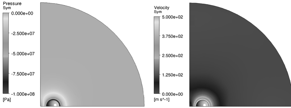
Fig. 4 CFD simulations showing the velocity field (on the right) causally associated with the pressure gradient around a vortex-particle attracting the DS. From it we can have an absorption velocity v_a in any point of the field.
