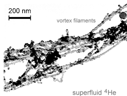
Fig. 1 Metallic nano-particles adhere onto vortex-filaments in superfluid ^4\text{He} making them visible, thanks to Bernoulli pressure [23, 24]. The attraction of the surrounding quanta in the DS exerted by vortex-particles is by us indicated as the quantum mechanism of gravity.
