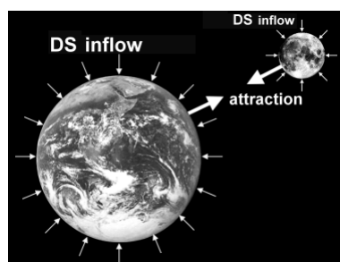
Fig. 2 Since macroscopic bodies consist of fundamental particles, they also produce a pressure gradient which becomes strong and evident around large celestial bodies, in which case we use the term “gravitational field”.
