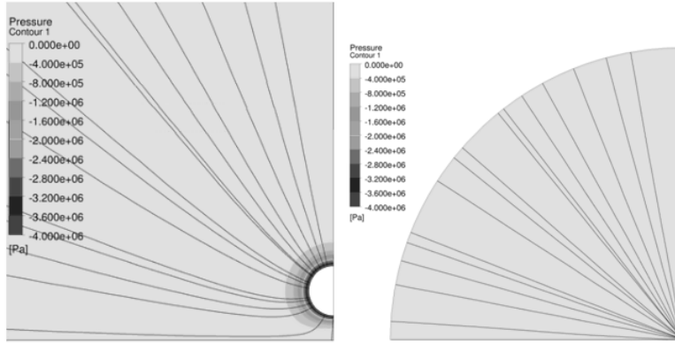
Fig. 3 CFD simulation putting in evidence the pressure gradient around a macroscopic spherical body absorbing the fluid in which it is immersed. The consequent 1/r^2 attractive force mathematically equals Gauss's law for gravity and is compatible with the Schwarzschild solution. Refining the grid (on the right) leads to a perfect radial simmetry.
