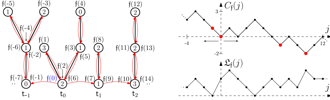
Figure 6: Contour and label functions C_{\mathbf{f}} and \mathfrak{L}_{\mathbf{f}} of an element ((\mathbf{f}, \mathfrak{l}), \mathbf{b}) \in \mathfrak{F}_{\infty} \times \mathfrak{B}_{\infty} . The left side depicts the two-sided contour exploration of \mathbf{f} . The labels are given by \mathfrak{L}_{\mathbf{f}}(j) , where now j \in \mathbb{Z} . The values of the infinite bridge \mathbf{b} at its first three down-steps to the right of 0 read here \mathbf{b}(d^{\downarrow}(1)) = 2 , \mathbf{b}(d^{\downarrow}(2)) = 1 and \mathbf{b}(d^{\downarrow}(3)) = 3 , while the first down-step to the left of zero has value \mathbf{b}(d^{\downarrow}(-1)) = 0 . The arrows below the contour function indicate the direction of the encoding, and the red dots mark again the encoding of a new tree.
