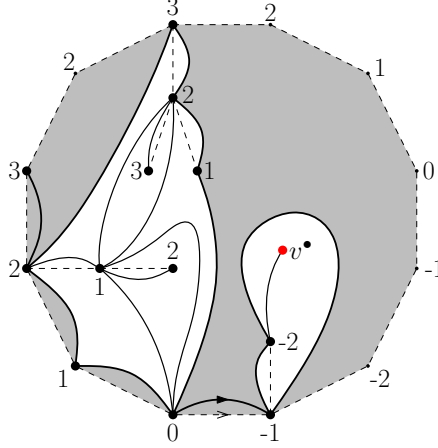
Figure 7: A representation of an element ((f, \ell), \mathbf{b}) \in \mathfrak{F}_6^6 \times \mathfrak{B}_6 in the plane and the associated rooted pointed quadrangulation (\mathbf{q}, v^\bullet) = \Phi_n((f, \ell), \mathbf{b}) . The distinguished vertex of the cycle is the down-most vertex labeled 0. The trees are grafted to the 6 down-steps of \mathbf{b} (here, d^\downarrow(1) = 0 , d^\downarrow(2) = 1 , d^\downarrow(3) = 8 , d^\downarrow(4) = 10 , d^\downarrow(5) = 11 , and d^\downarrow(6) = 12 ). The tree edges are indicated by the dashed lines in the interior of the cycle. Note that three trees (those above the first, fourth and sixth down-step) consist of a single vertex. The labels in a tree are shifted by the bridge value of the down-step above which the tree is attached. Note that the 12 boundary edges of the cycle are in an order-preserving correspondence with the 12 boundary edges of \mathbf{q} . (The two edges of \mathbf{q} which lie entirely in the outer face are counted twice.)
