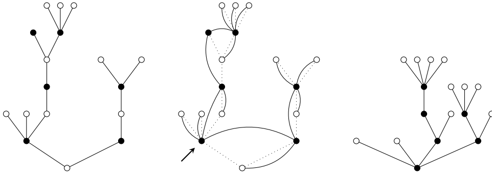
Figure 4: The Janson–Stefansson bijection from two-type trees to one-type trees.
