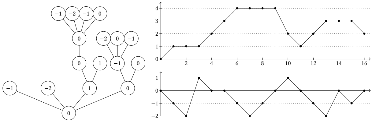
Figure 2: A one-type labelled tree, its height process on top and its label process below.
