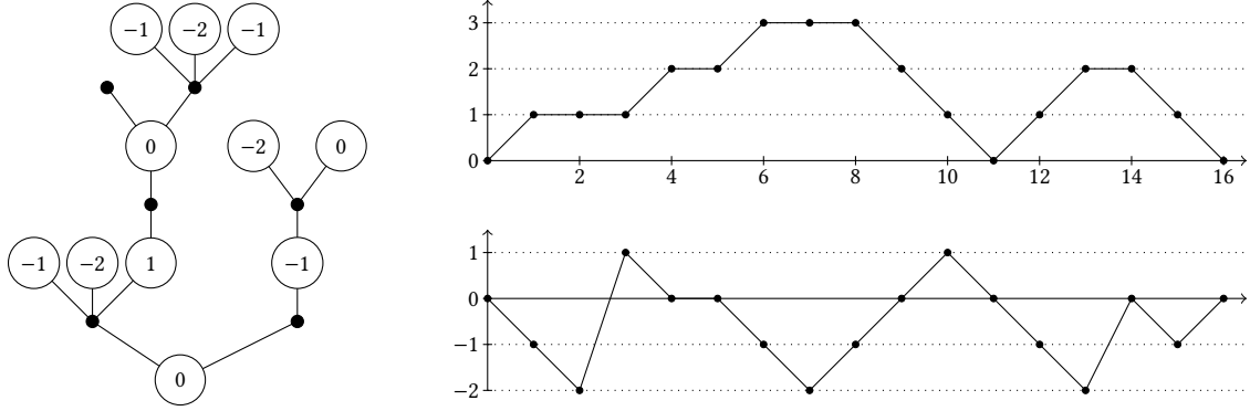
Figure 1: A two-type labelled tree, its white contour process on top and its white label process below.
