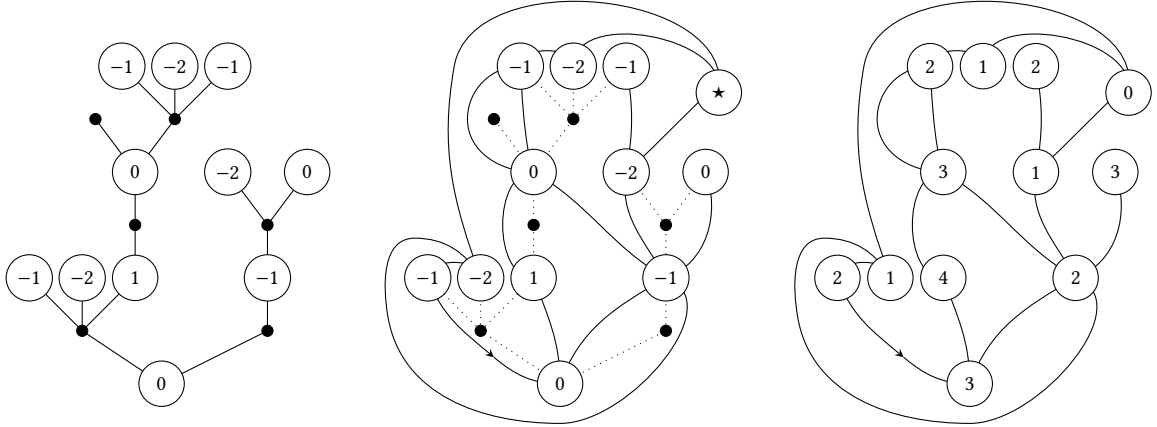
Figure 3: The Bouttier–Di Francesco–Guitter bijection.
