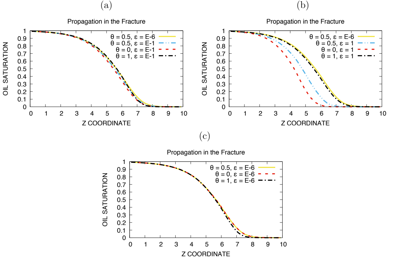
Figure 5: Fracture oil saturation for time t = 6h .
