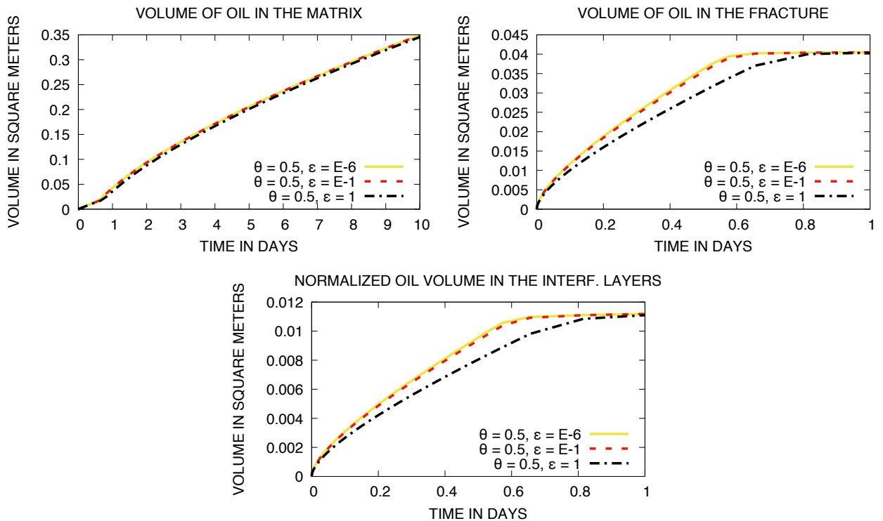
Figure 6: Volume occupied by oil in the matrix, fracture and oil volume normalised by \varepsilon in the interfacial layers, for \theta = 0.5 , as a function of time.
