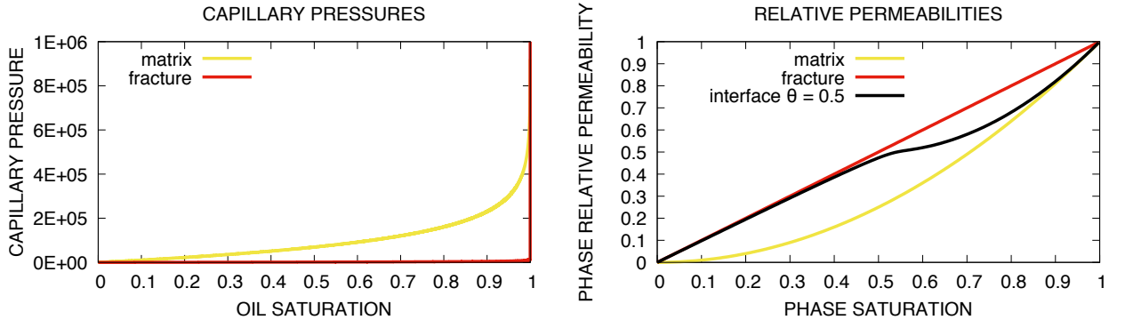
Figure 4: Curves for capillary pressures and relative permeabilities.
