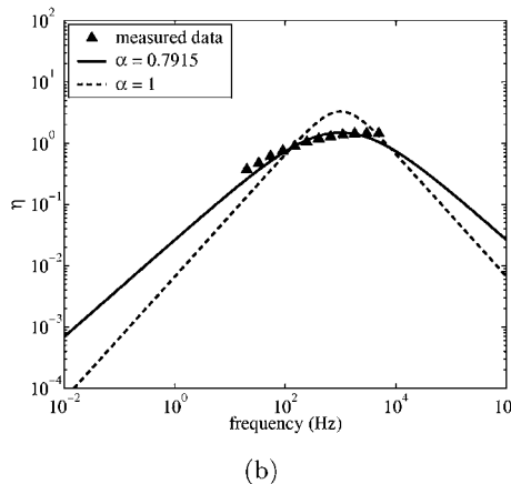
Fig. 1. Master curves of 3M ISD112 viscoelastic material at 27°C: a Storage modulus G' and b loss factor \eta
