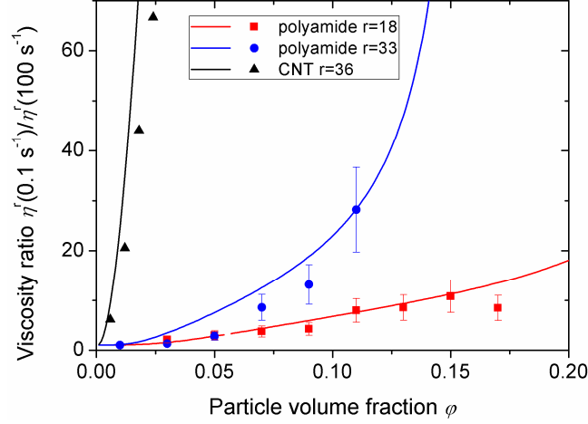
Fig. 10. Theoretical and experimental dependences of the ratio of low-shear-to-high-shear viscosity \eta^r(0.1 \text{ s}^{-1})/\eta^r(100 \text{ s}^{-1}) on particle volume fraction. Symbols – experiment, solid lines – theory. The values of the adjustable parameters are summarized in Table IV of Appendix D.
