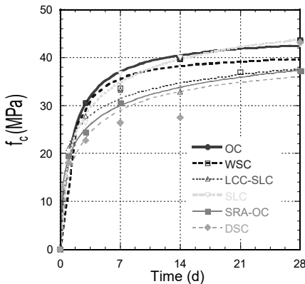
Figure 4: Compressive strength evolution.
