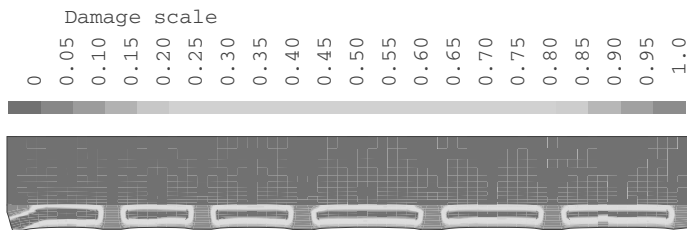
Figure 14: Damage due to restrained shrinkage in repaired beam
