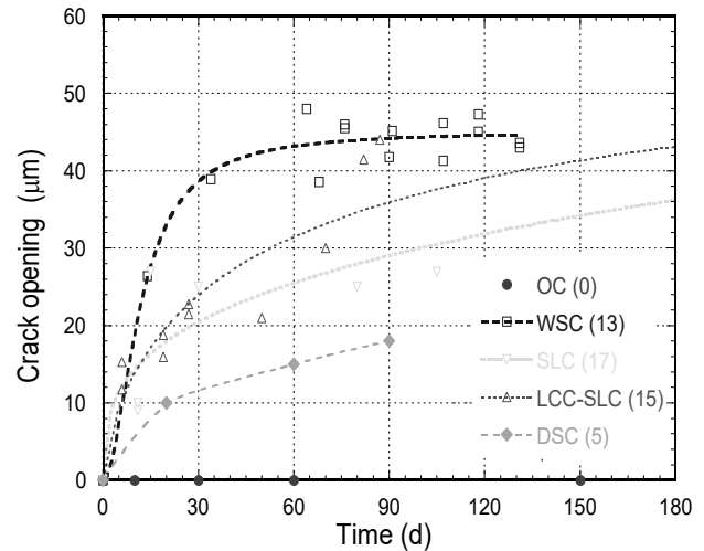
Figure 9: Crack width evolution - Drying only.
