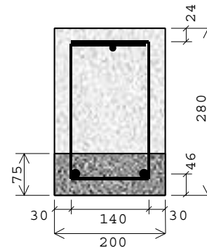
Figure 3: Section of test beams.
