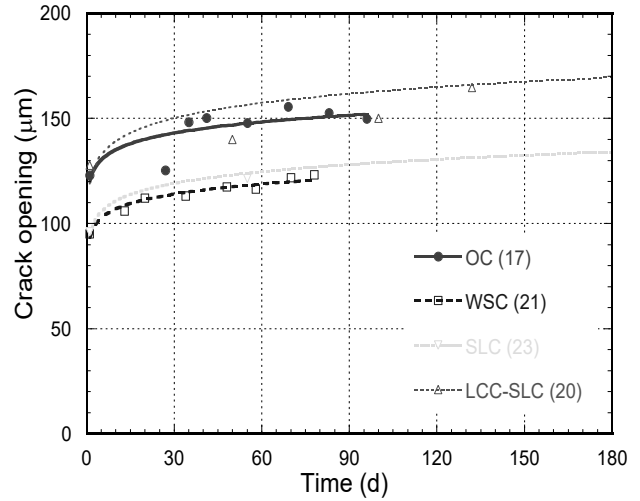
Figure 12: Crack width evolution - Loaded at 66%.
