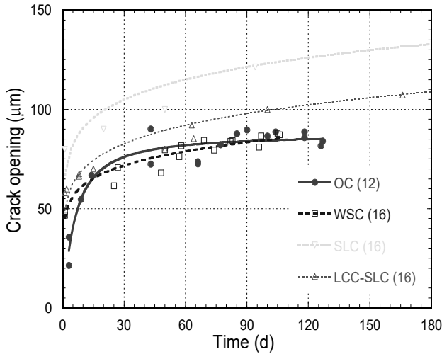
Figure 11: Crack width evolution - Loaded at 33%.
