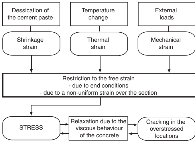
Figure 1: Schematical illustration of the stress build-up in repairs (Saucier et al. 1997).
