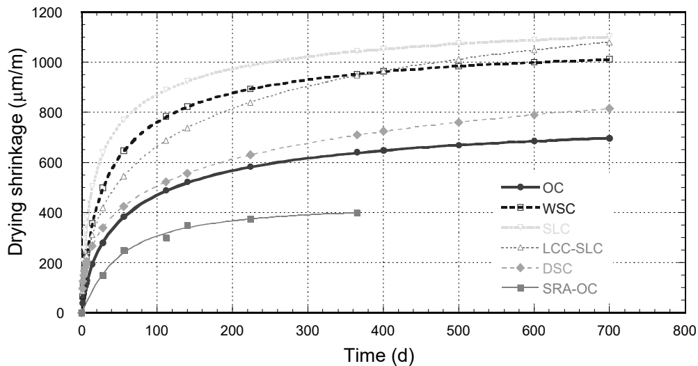
Figure 6: Drying shrinkage.
