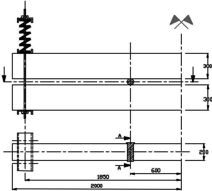
Figure 10: Loading setup
