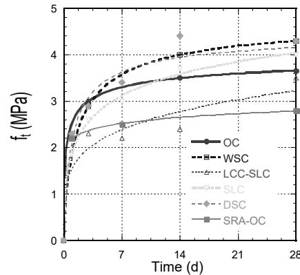
Figure 5: Tensile strength evolution.
