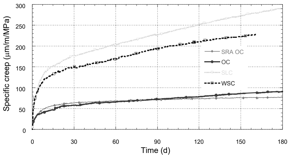
Figure 7: Specific tensile creep.
