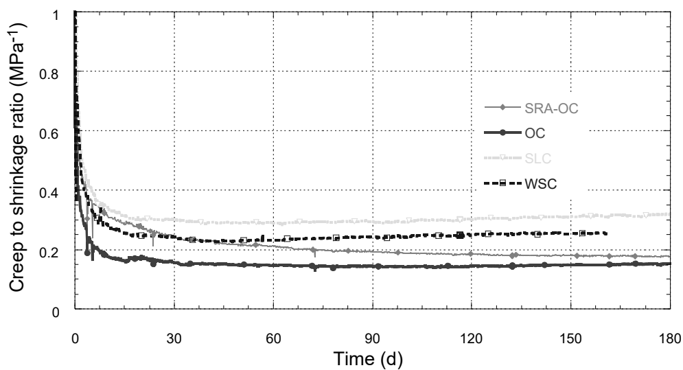
Figure 8: Specific creep to shrinkage ratio.
