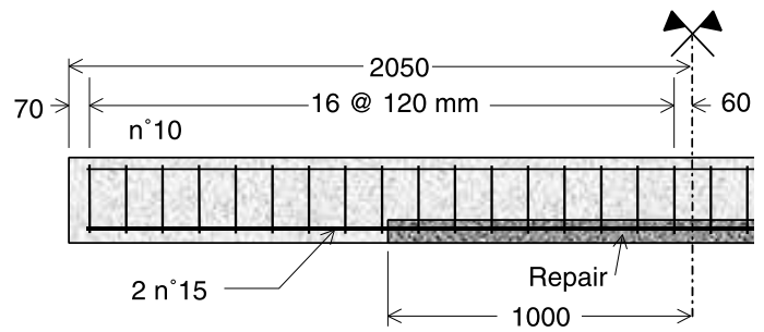
Figure 2: Test specimens.
