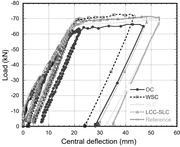
Figure 13: Flexural testing (drying only series).
