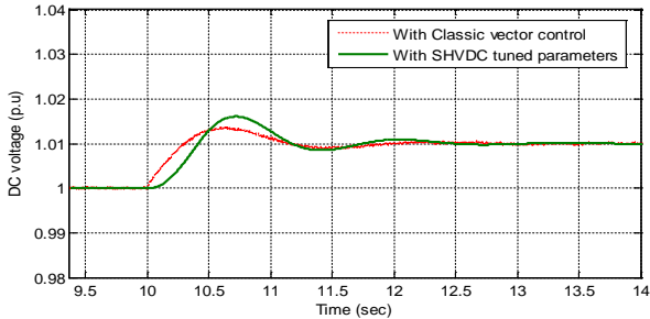
Fig. 7. Responses with optimal parameters. (a) Response of P_g to a +0.05 step in P_{g\_ref} (p.u.) ; (b) Response of Q_g to a -0.1 step in Q_{g\_ref} (p.u.); (c) Response of V_g to a -0.1 step change in Q_{g\_ref} (p.u.); (d) Response of V_m to -0.1 step change in Q_{m\_ref} (p.u.); (e) Response of V_{dc} to a +0.01 step in V_{dc\_ref} (p.u.).
