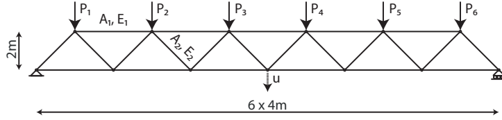
Figure 17: Two-dimensional truss – geometry, loading and QoI
