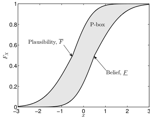
Figure 1: Probability-boxes
