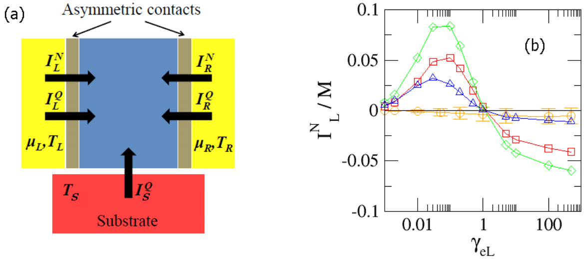
Figure 5: (a) : Scheme of the three-terminal setup corresponding to activated thermoelectric transport for a NW deposited on a substrate. The NW (blue) is connected to two electronic electrodes (yellow) L (the source) and R (the drain) via asymmetric contacts. The electrodes are at equilibrium (electrochemical potentials \mu_L , \mu_R , and temperatures T_L , T_R ). The insulating substrate (red) provides a phonon bath of temperature T_S . (b) : Ratchet effect powered by \delta T_S = 10^{-3} \epsilon when \delta T = \delta \mu = 0 . For various values of V_g ( V_g/\epsilon = 0 ( \circ ), 0.5 ( \square ), 1 ( \diamond ) and 2.5 ( \triangle )), the average particle currents I_L^N/M (in unit of 10^5 \epsilon/\hbar ) of an array of M = 2 \cdot 10^5 parallel NWs is given as one varies \gamma_{eL} (elastic coupling to the source), keeping the same value \gamma_{eR} = \epsilon/\hbar for the elastic coupling to the drain. I_L^N/M \neq 0 , unless V_g = 0 (particle-hole symmetry) or \gamma_{eL} = \gamma_{eR} (inversion symmetry).
