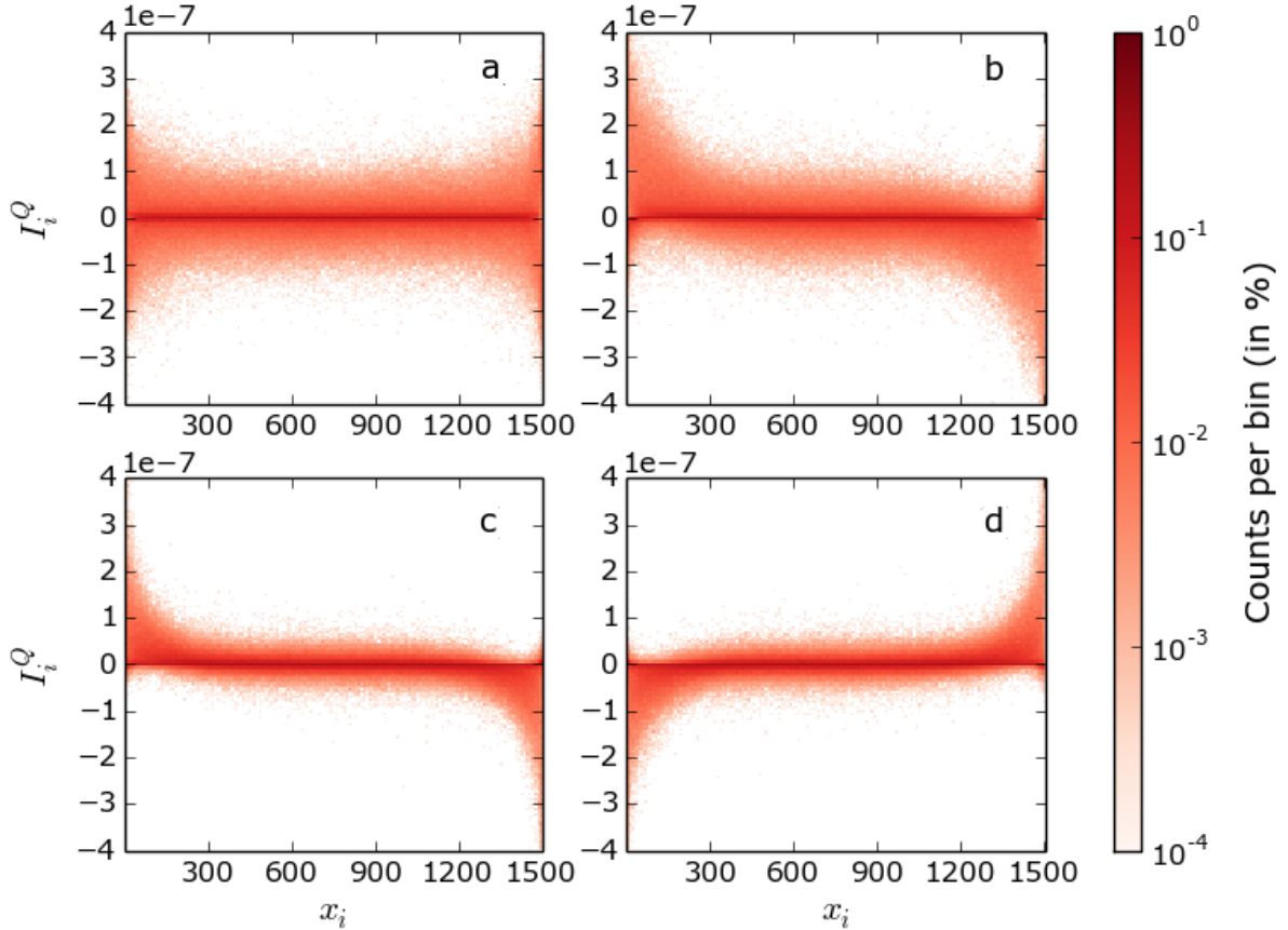
Figure 4: 2D histograms giving the distribution of local heat currents I_i^Q (Eq. (19)) as a function of the position x_i along the NW, for four values of the gate potential: (a) V_g = 0 , (b) V_g = t , (c) V_g = 2.25t and (d) V_g = -2.25t . Parameters: L = 1500 , W = t , k_B T = 0.1t , \delta\mu = 10^{-5}t , statistics over 500 NWs.
