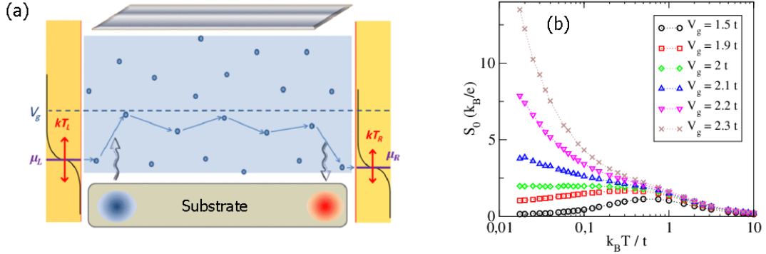
Figure 3: (a) The electronic localised states (blue dots) are randomly located along the chain within an energy band of width 4t+W (shaded light blue region). In the left and right reservoirs, the electrons are at equilibrium with Fermi-Dirac distributions of temperatures T_L = T + \delta T , T_R = T and electrochemical potentials \mu_L = E_F + \delta\mu , \mu_R = E_F . Varying the voltage V_g applied to the gate (top grey region) shifts the NW conduction band, making possible to probe electron transport inside the band, around its edges or outside the band. The electrons can hop between states of different energies by absorbing or emitting a phonon. For a NW deposited on a substrate, the phonons are provided by the substrate and characterized by a Bose-Einstein distribution of temperature T_S ( T_S = T throughout the paper, except in Sec.5). Electrons injected near the lower band edge mainly find available states to jump to at higher energies near the source (left reservoir). This implies that the phonons are mainly absorbed from the substrate near the source (blue region), and emitted back to the substrate near the drain (red region), as indicated by the two arrows. (b) Typical thermopower S_0 (in units of k_B/e ) as a function of k_B T/t , calculated for a chain of length L = 200 ( E_F = 0 and W = t ) for increasing values of V_g .
