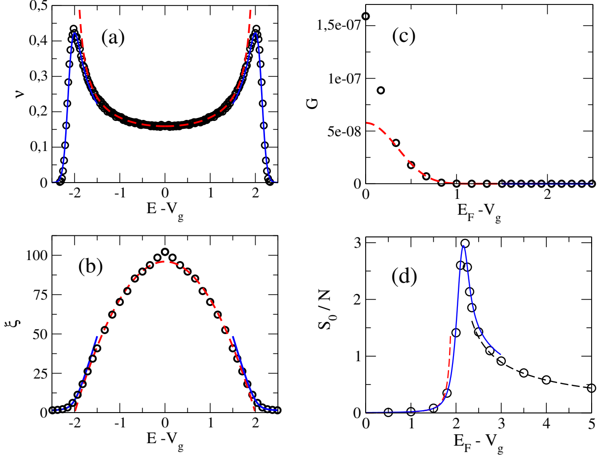
Figure 2: 1D Anderson model with W = t = 1 : (a) Density of states per site \nu(E) , (b) localization length \xi(E) , (c) typical conductance G (in units of 2e^2/h ) and (d) typical thermopower S_0 (in units of (\pi^2 k_B)/(3e)k_B T ). In all panels, the red dashed line and the blue continuous line give the weak disorder behaviours in the bulk and near the edges (Eqs. (3-5) and Eqs. (8-9)), while the black dashed line in (d) corresponds to Eq. (10). Circles are numerical results obtained for N = 1600 ((a) and (b)) and N = 800 ((c) and (d)).
