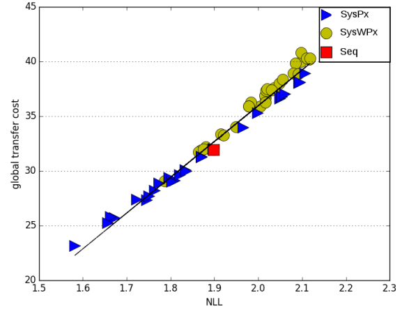
Figure 9. Graph of average transport cost, function of average NLL on 45 sequences corpus for Seq , SysP0 ...29 and SysWP0 ...29.
