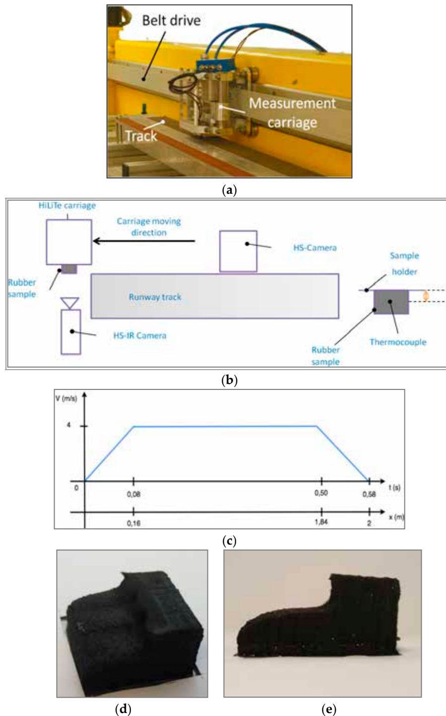
Figure 2. (a) High Speed Linear Tester (HiLiTe); (b) test set-up for contact temperature and deformation measurements; (c) test phases; (d,e) final sample shape after sliding phase on concrete test track.
