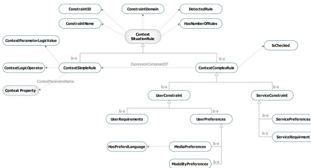
Figure 10. Context constraint sub-ontology.
