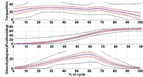
Figure 7: Mean and Standard deviation plots for velocity, position and torque in flexion Phase for all subjects
