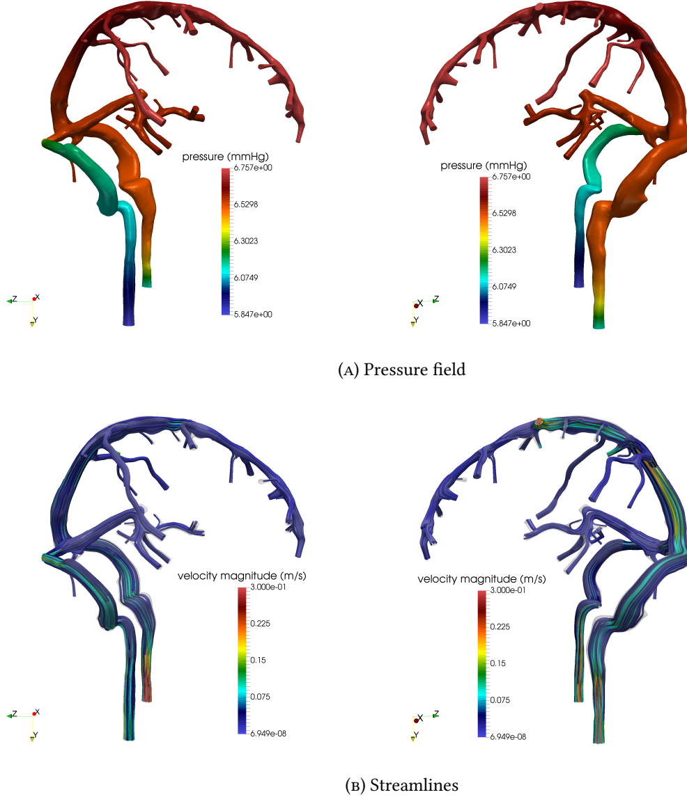
FIGURE 6. Cerebral venous hemodynamics obtained by imposing a pressure drop between the inlet and outlet sections
