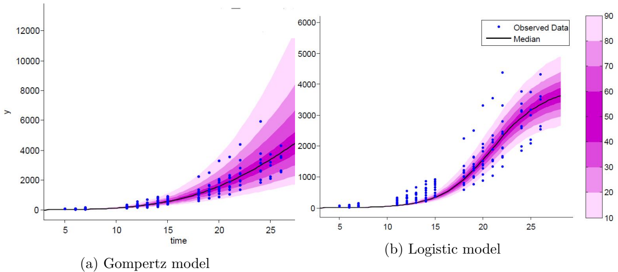
Figure 4: Prediction distribution on Monolix
