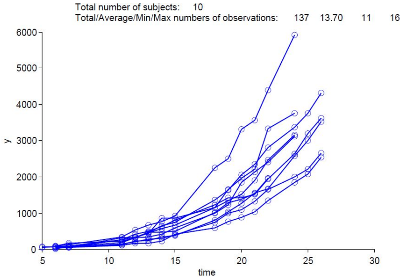
Figure 1: Volume of tumor data for 10 mice with Monolix
