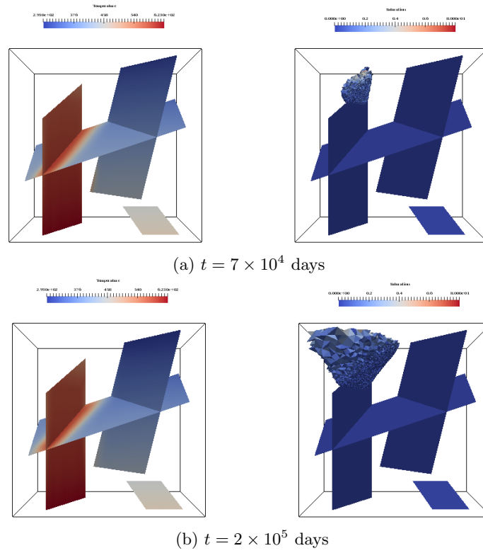
Figure 18: Left: temperature in the faults at different times (days). Right: saturation of gas in the faults and in the matrix domain at different times (days) where a threshold of 0.0001 is used on the matrix domain.
