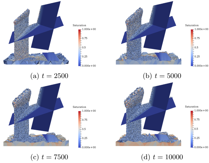
Figure 9: Oil saturation in the fractures and in the matrix domain at different times (in days) for the tetrahedral mesh. A threshold of 0.2 is used for the saturation in the matrix domain.
