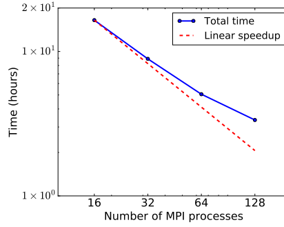
Figure 7: Total computation time vs. number of MPI processes for the two phase immiscible isothermal flow test case with hexahedral mesh where n_x = 128 .
