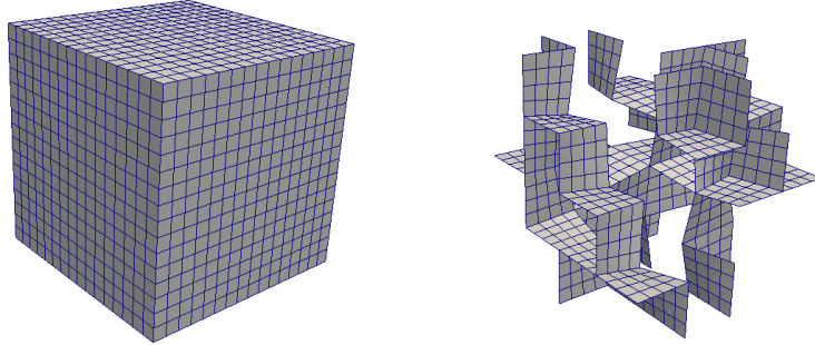
Figure 5: Example of hexahedral mesh of the matrix domain (left) conforming to the fracture network (right) where n_x = 16 .
