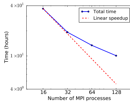
Figure 19: Total computation time vs. number of MPI processes for the thermal convection test with tetrahedral mesh.
