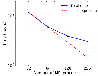
Figure 15: Total computation time vs. number of MPI processes for the non-isothermal test case on the prismatic mesh.
