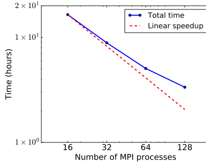
Figure 7: Total computation time vs. number of MPI processes for the two phase immiscible isothermal flow test case with hexahedral mesh where n_x = 128 .
