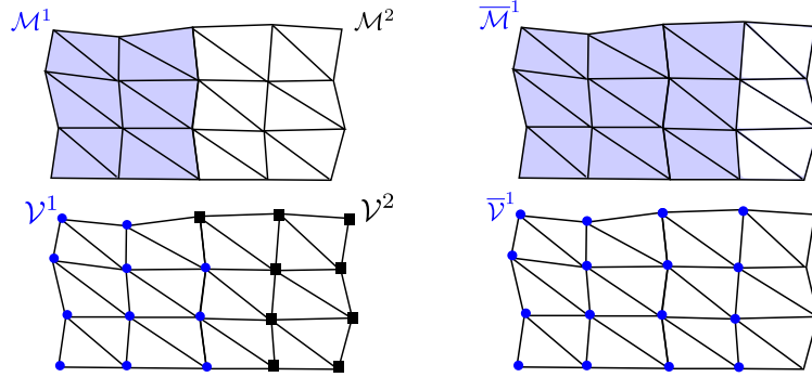
Figure 4: Example of mesh decomposition.
