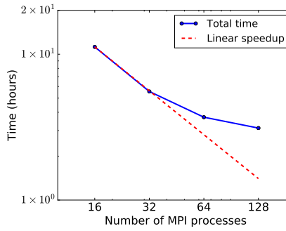
Figure 11: Total computation time vs. number of MPI processes for the black oil model test case with tetrahedral mesh.
