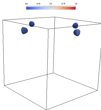
Figure 17: Saturation of gas in the matrix domain at the final time t_f = 2 \times 10^7 days.
