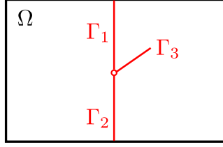
Figure 1: Example of a 2D domain with 3 intersecting fractures \Gamma_1, \Gamma_2, \Gamma_3 .
