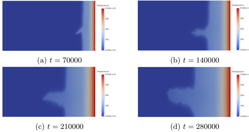
Figure 13: Temperature in the matrix domain for the non-isothermal test case on the prismatic mesh.
