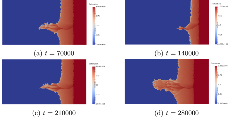
Figure 14: Gas saturation in the matrix domain for the non-isothermal test case on the prismatic mesh.
