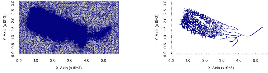
Figure 12: 2D view of prismatic mesh of the matrix domain (left) conforming to the fault network (right).
