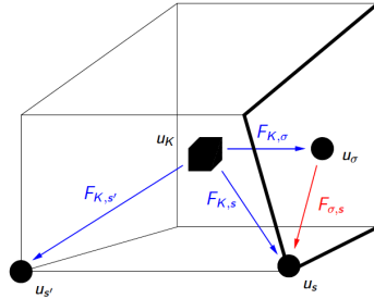
Figure 2: For a cell K and a fracture face \sigma (in bold), examples of VAG degrees of freedom u_K, u_{\mathbf{s}}, u_{\sigma}, u_{\mathbf{s}'} and VAG fluxes F_{K,\sigma}, F_{K,\mathbf{s}}, F_{K,\mathbf{s}'}, F_{\sigma,\mathbf{s}} .
