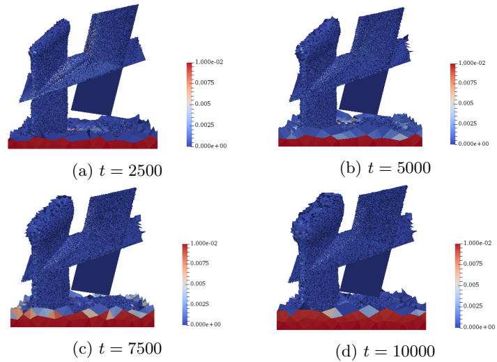
Figure 10: Molar fraction of the HC component in the water phase in the fractures and in the matrix domain at different times (in days) for the tetrahedral mesh. A threshold of 0.001 is used for the saturation in the matrix domain.
