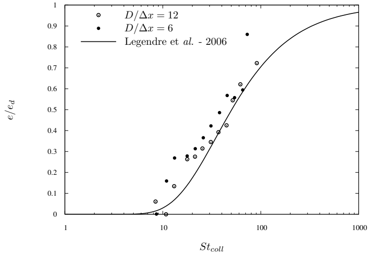
Figure 1: Normal restitution coefficient of collisions with respect to collisional Stokes number St_{coll} = \frac{2}{9} \frac{R^{u_{coll}pp}}{\mu_f} : influence of the spatial resolution.
