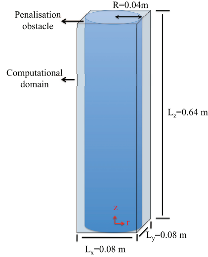
Figure 2: Geometry and dimensions of the computational domain.
