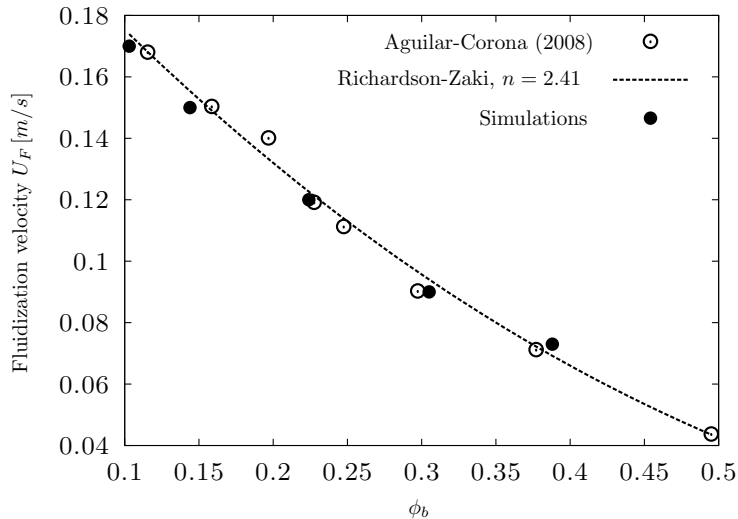
Figure 6: Fluidization velocity with respect to the bed solid concentration. \odot : Aguilar-Corona (2008), - - - : (Richardson and Zaki, 1954)’s correlation with n = 2.41 and \bullet : present simulations.
