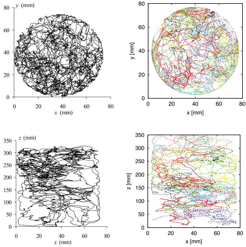
Figure 7: Projections of particle trajectories in x - y plane (top) and x - z plane (bottom). Left: Experimental data by Aguilar-Corona (2008) ( U_F = 0.15 m/s, \phi_b = 0.14 ), right: Simulations.
