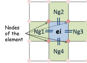
Figure 1: Representation of a mesh element ei and its neighbors in 2D
