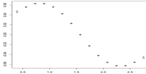
Figure 3: Approximation of the driver at t = T with only three local polynomials - Crosses: f(\cdot, \cos) . Circles: f_{\ell_o}(\cdot, \cos, \cos) .
