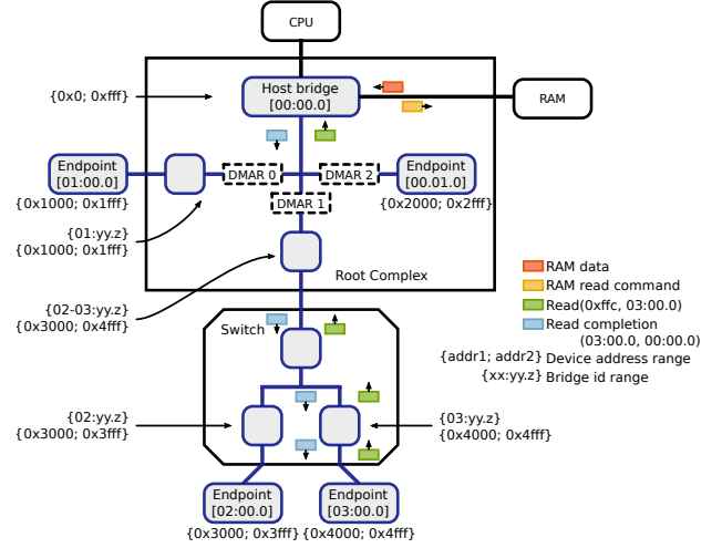
Fig. 2. Memory read message routing
