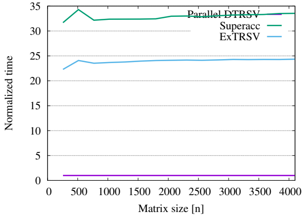
(a) \ln TRSV on K20c
