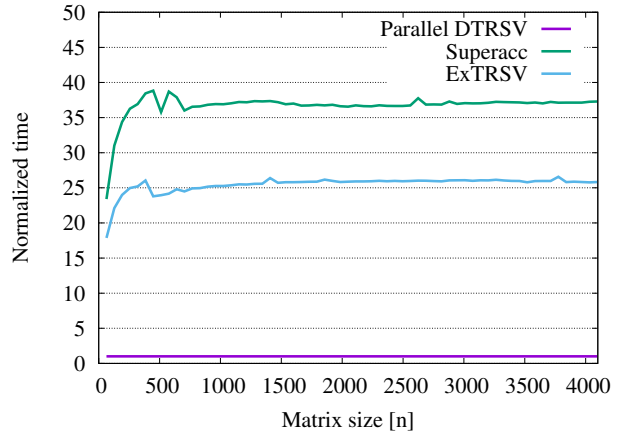
(b) \ln TRSV on K80
