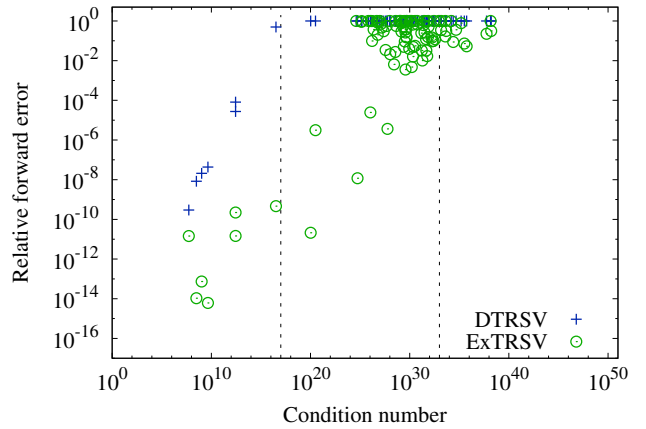
(d) Accuracy of TRSV with respect to the condition number of the matrix A
