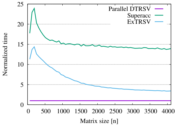
(c) \ln TRSV on K420
