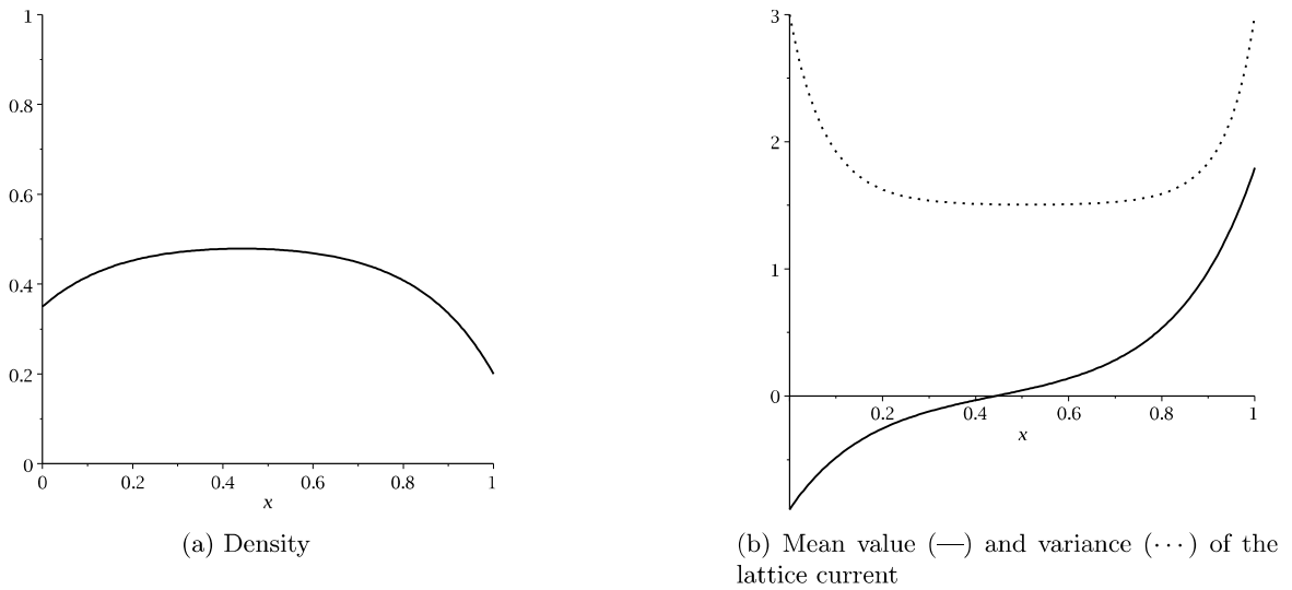
Figure 3: Plot of the density and of the lattice current for \rho_a = 0.35 , \rho_b = 0.2 and \lambda_0 = 3 .
