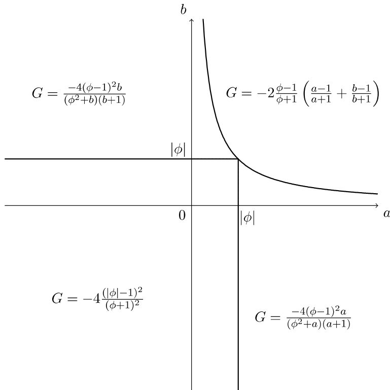
Figure 6: Value of the gap G depending on the parameters a , b and \phi . The equation of the curve is b = \phi^2/a . (This particular figure is drawn for \phi = 1/4 ( \lambda = 0.6 ) even though similar one is valid for any \phi ).
