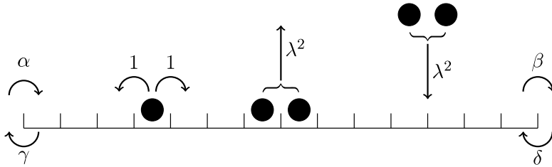
Figure 1: Dynamical rules of the model.
