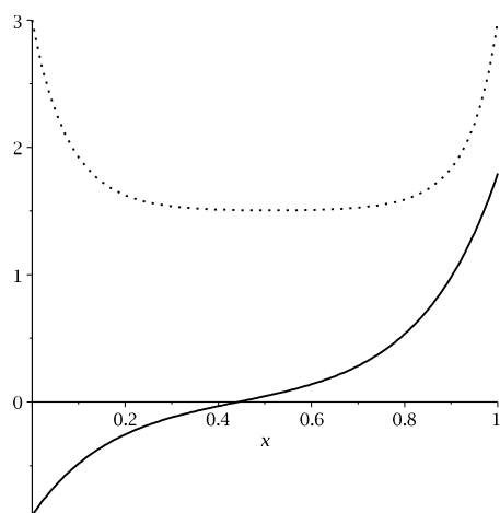
(b) Mean value (—) and variance (···) of the lattice current
