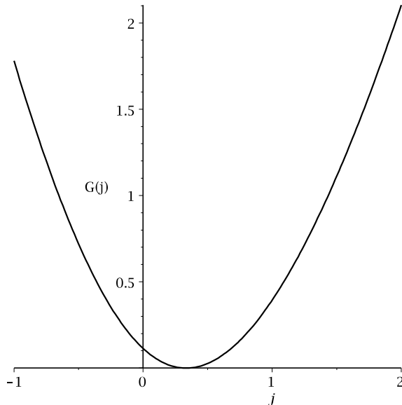
Figure 2: Example of large deviation function G(j) (on the plot \alpha = 2, \gamma = 0.5 ).
