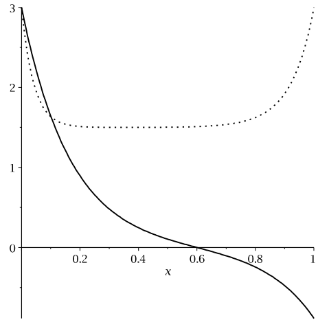
(b) Mean value (—) and variance ( \cdots ) of the lattice current
