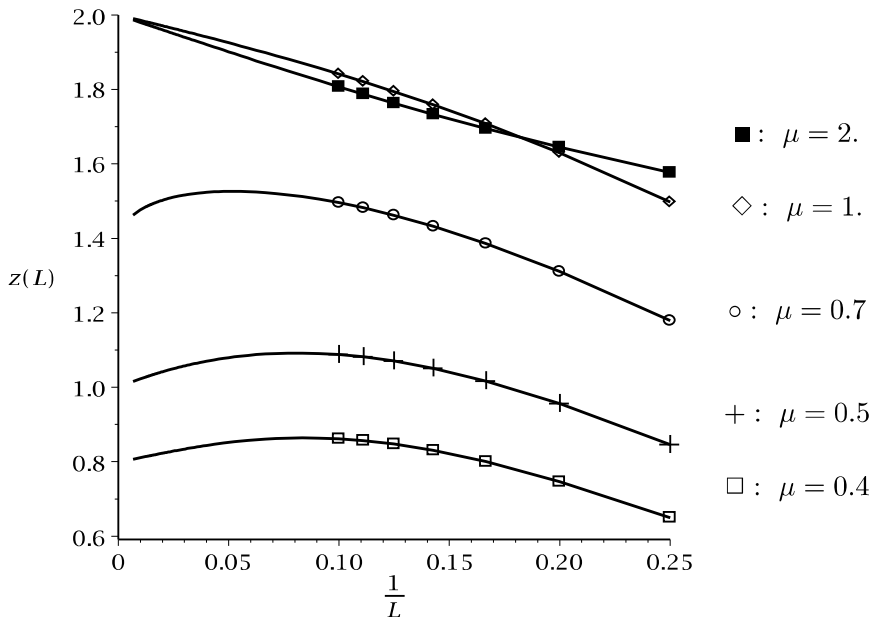
Figure 7: Behavior of the gap in the thermodynamic limit when \lambda behaves as \frac{1}{L^\mu} : plot of z(L) = \frac{\ln(G_L) - \ln(G_{L-1})}{\ln(L-1) - \ln(L)} as a function of \frac{1}{L} . The lines represent the values obtained from Bethe ansatz (for 4 \leq L \leq 150 ), while the dots correspond to direct diagonalisation of H (for 4 \leq L \leq 10 ).
