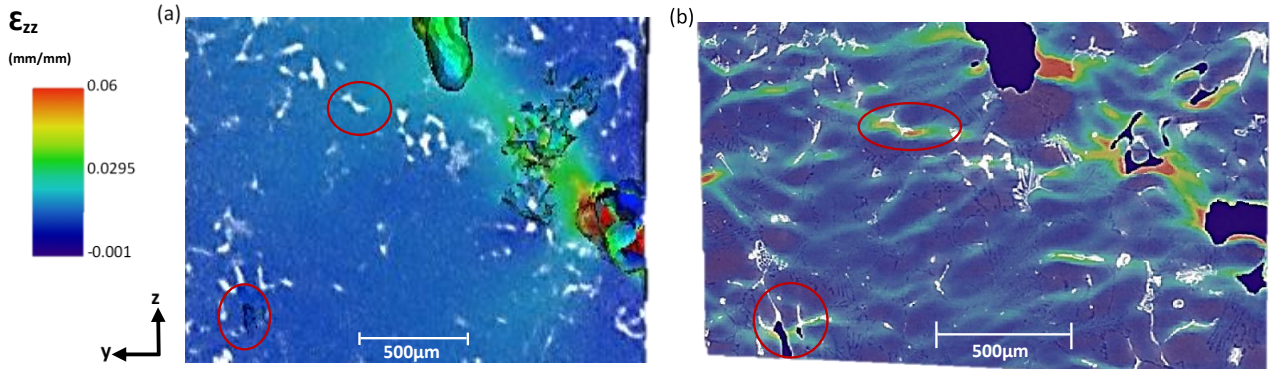
Figure 10: Comparison between FE calculations and DVC results in the bulk at 250°C, \sigma_{max} = 75 \text{ MPa} (a) Strain field computed by FE simulation during monotonic loading (elasto plastic calculation), i.e. at the maximum load of the first half-cycle of fatigue and (b) Strain field measured with DVC between the minimum and maximum of the first cycle; strain localization at hard second phase particles in the DVC results are circled in red.
