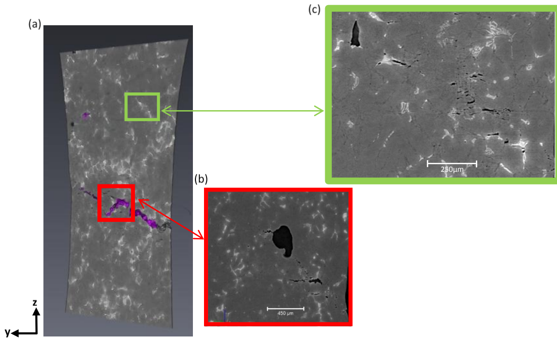
Figure 9: Observation of cracks in the specimen at 250°C at a tomography image at 610 \mu m below the surface, \sigma_{max} = 75MPa: (a) before failure (40th cycle), (b) failure zone and (c) far away from the principal crack
